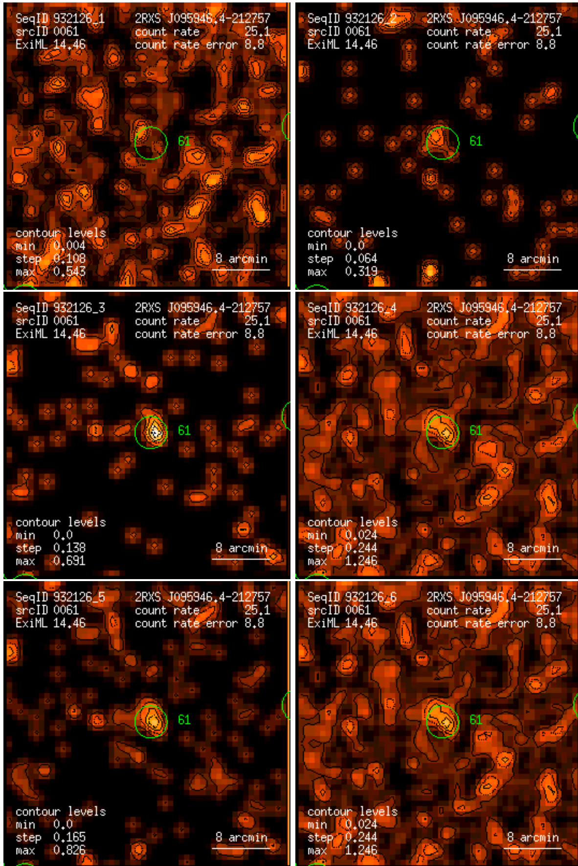
Figure 61: RASS 932126: detection 0061: band rate images, Gaussian filter: (1) PSPC channels 11 – 41, (2) 52 – 90, (3) 91 – 201, (4) 11 – 235, (5) 52 – 201, (6) 11 – 201. Broad band rates in counts/ks. Band rate contour levels in counts/ks/arcmin 2 .
