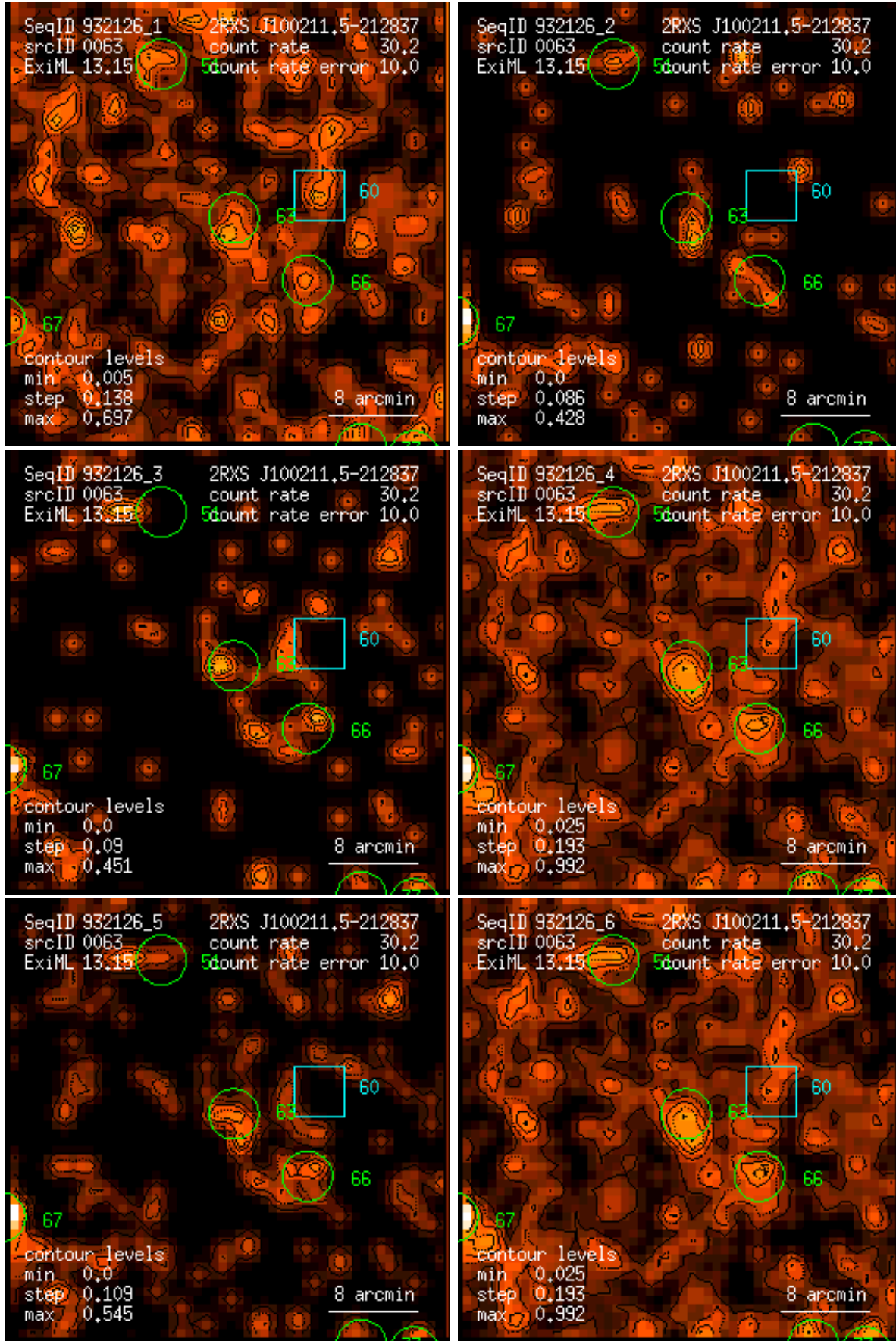
Figure 63: RASS 932126: detection 0063: band rate images, Gaussian filter: (1) PSPC channels 11 – 41, (2) 52 – 90, (3) 91 – 201, (4) 11 – 235, (5) 52 – 201, (6) 11 – 201. Broad band rates in counts/ks. Band rate contour levels in counts/ks/arcmin 2 .
