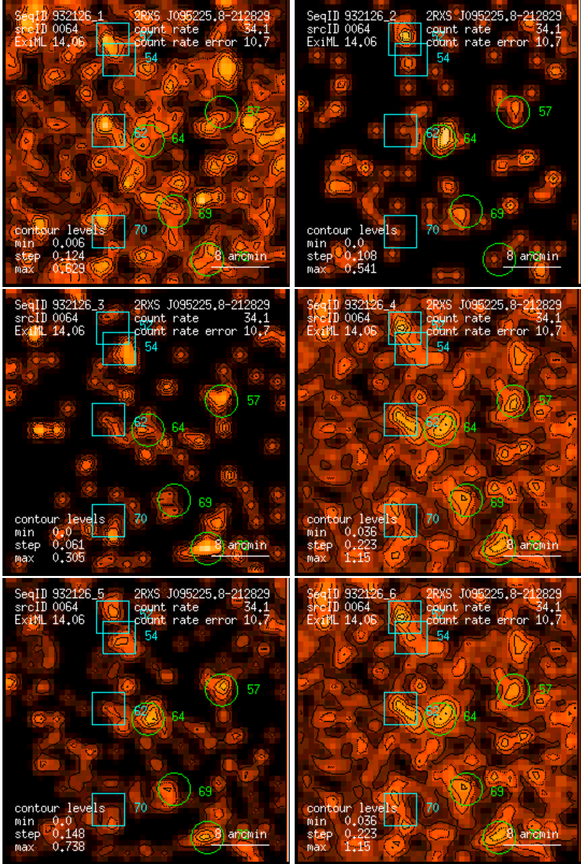
Figure 64: RASS 932126: detection 0064: band rate images, Gaussian filter: (1) PSPC channels 11 – 41, (2) 52 – 90, (3) 91 – 201, (4) 11 – 235, (5) 52 – 201, (6) 11 – 201. Broad band rates in counts/ks. Band rate contour levels in counts/ks/arcmin 2 .
