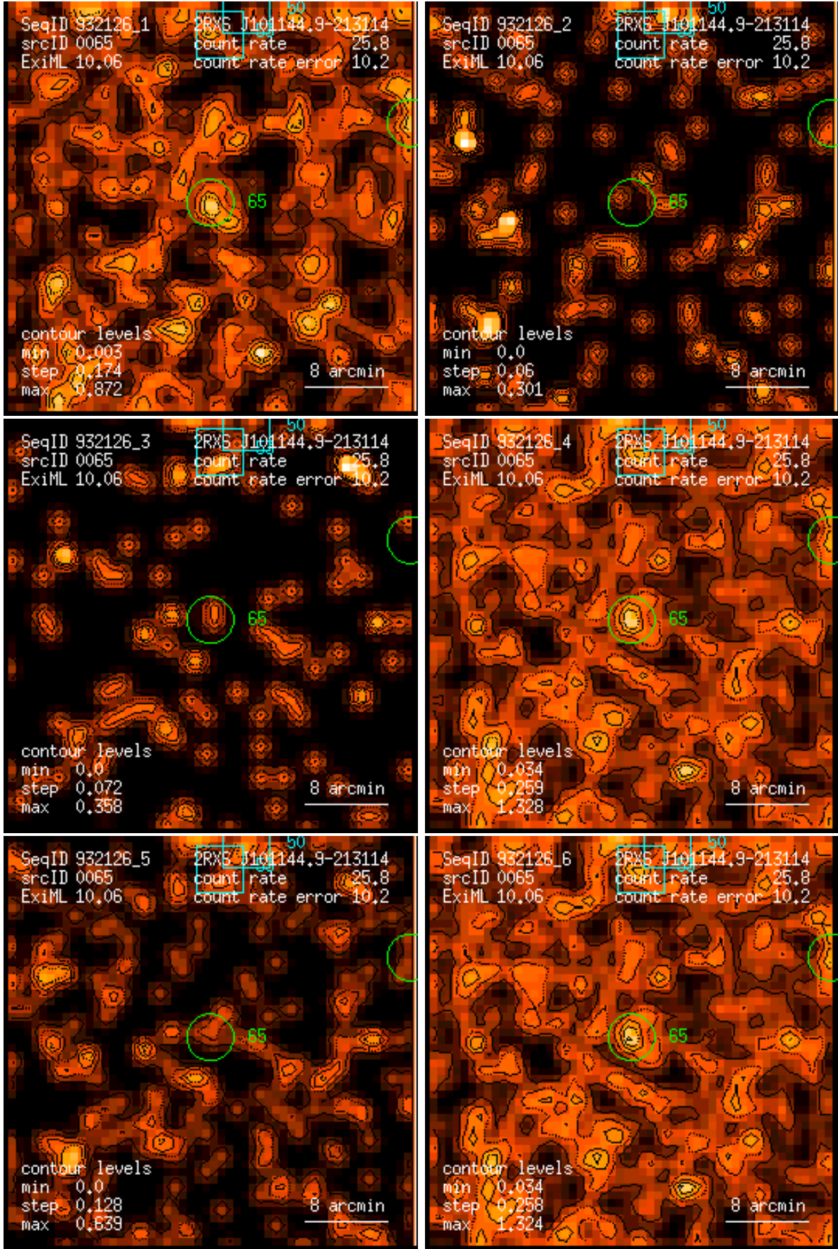
Figure 65: RASS 932126: detection 0065: band rate images, Gaussian filter: (1) PSPC channels 11 – 41, (2) 52 – 90, (3) 91 – 201, (4) 11 – 235, (5) 52 – 201, (6) 11 – 201. Broad band rates in counts/ks. Band rate contour levels in counts/ks/arcmin 2 .
