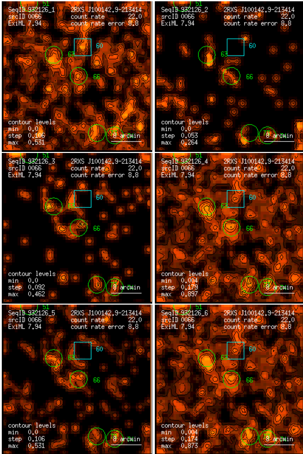
Figure 66: RASS 932126: detection 0066: band rate images, Gaussian filter: (1) PSPC channels 11 – 41, (2) 52 – 90, (3) 91 – 201, (4) 11 – 235, (5) 52 – 201, (6) 11 – 201. Broad band rates in counts/ks. Band rate contour levels in counts/ks/arcmin 2 .
