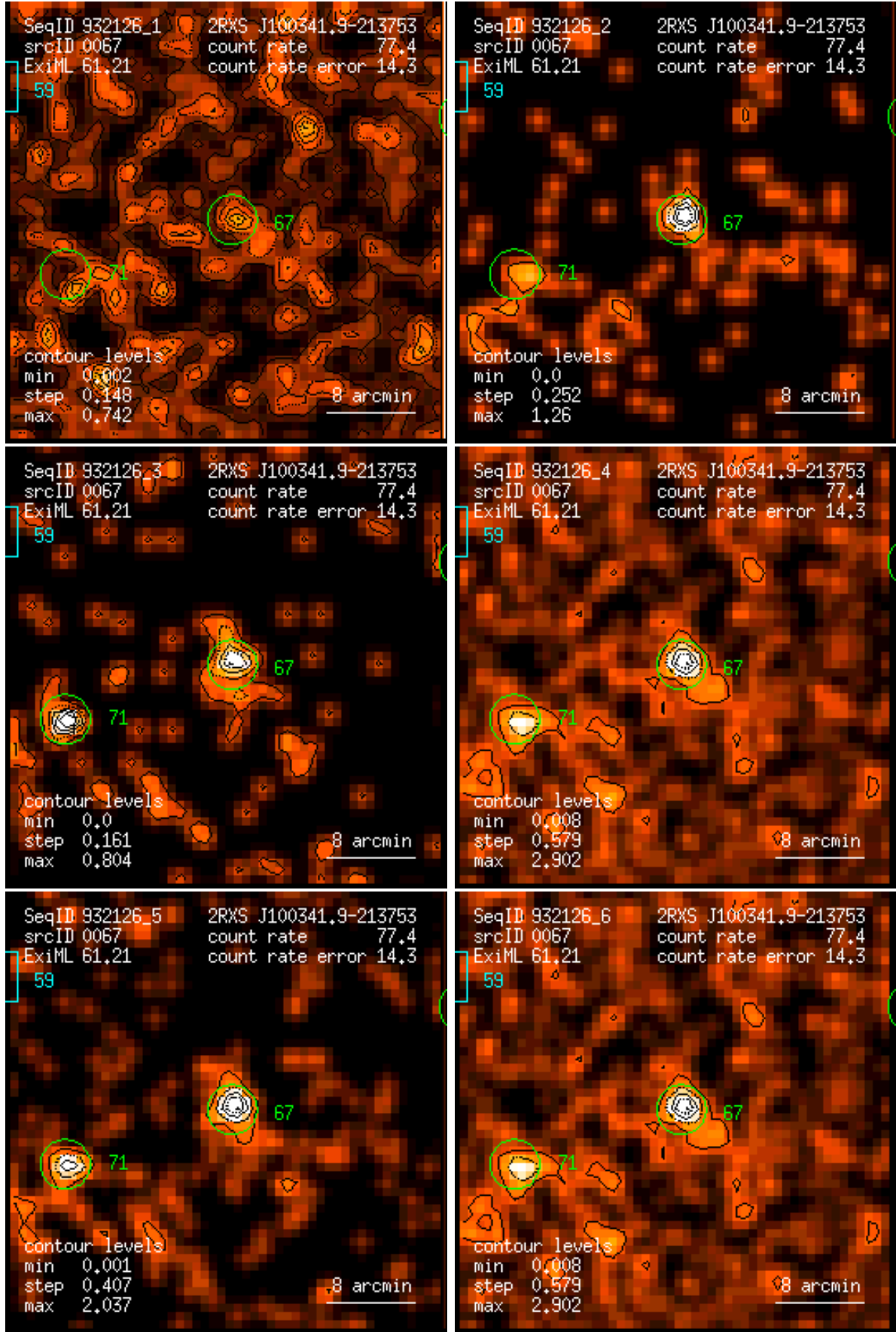
Figure 67: RASS 932126: detection 0067: band rate images, Gaussian filter: (1) PSPC channels 11 – 41, (2) 52 – 90, (3) 91 – 201, (4) 11 – 235, (5) 52 – 201, (6) 11 – 201. Broad band rates in counts/ks. Band rate contour levels in counts/ks/arcmin 2 .
