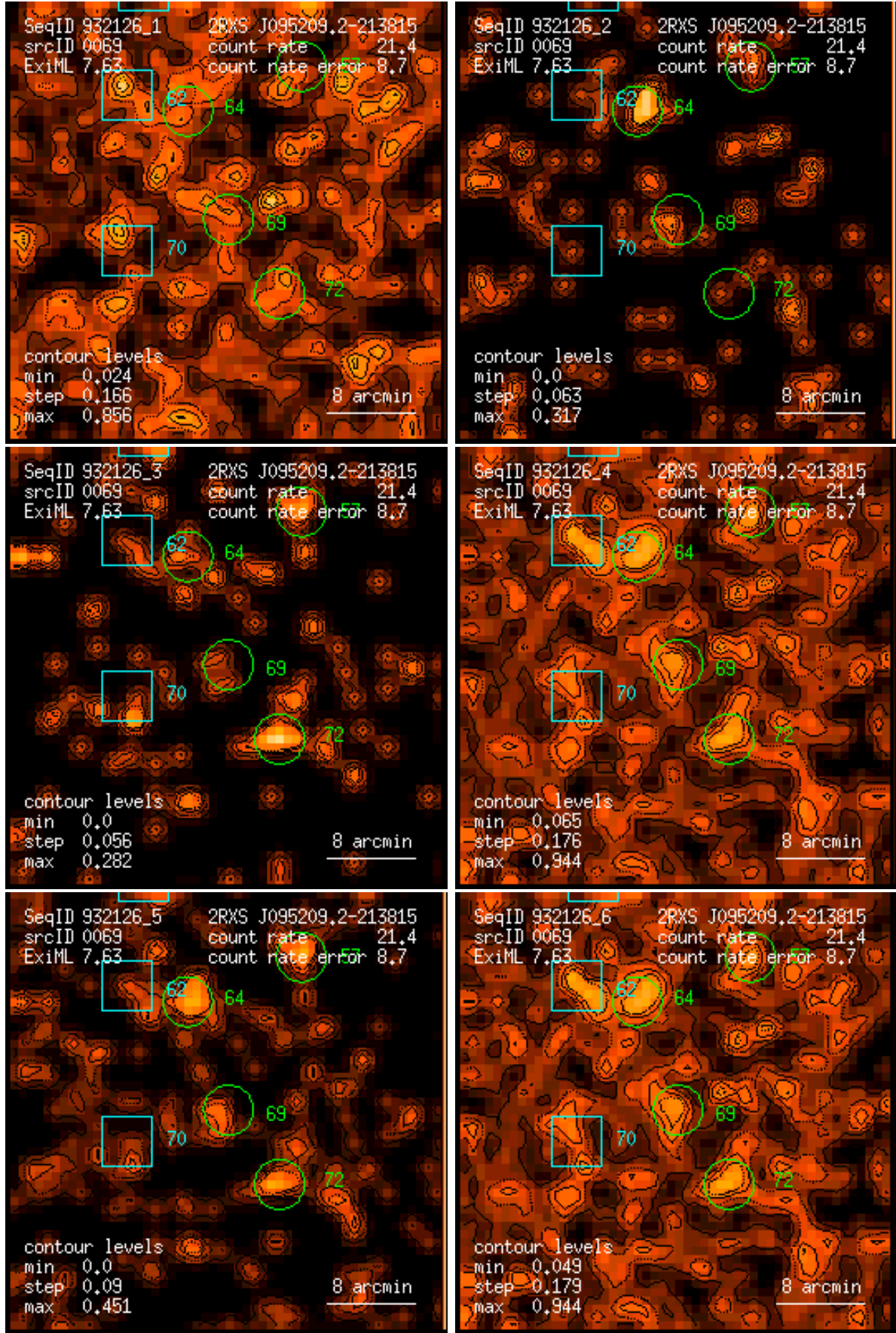
Figure 69: RASS 932126: detection 0069: band rate images, Gaussian filter: (1) PSPC channels 11 – 41, (2) 52 – 90, (3) 91 – 201, (4) 11 – 235, (5) 52 – 201, (6) 11 – 201. Broad band rates in counts/ks. Band rate contour levels in counts/ks/arcmin 2 .
