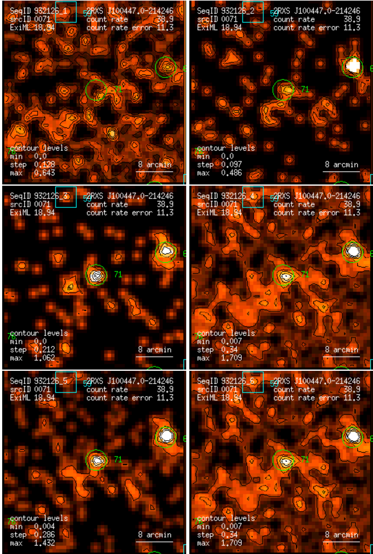
Figure 71: RASS 932126: detection 0071: band rate images, Gaussian filter: (1) PSPC channels 11 – 41, (2) 52 – 90, (3) 91 – 201, (4) 11 – 235, (5) 52 – 201, (6) 11 – 201. Broad band rates in counts/ks. Band rate contour levels in counts/ks/arcmin 2 .
