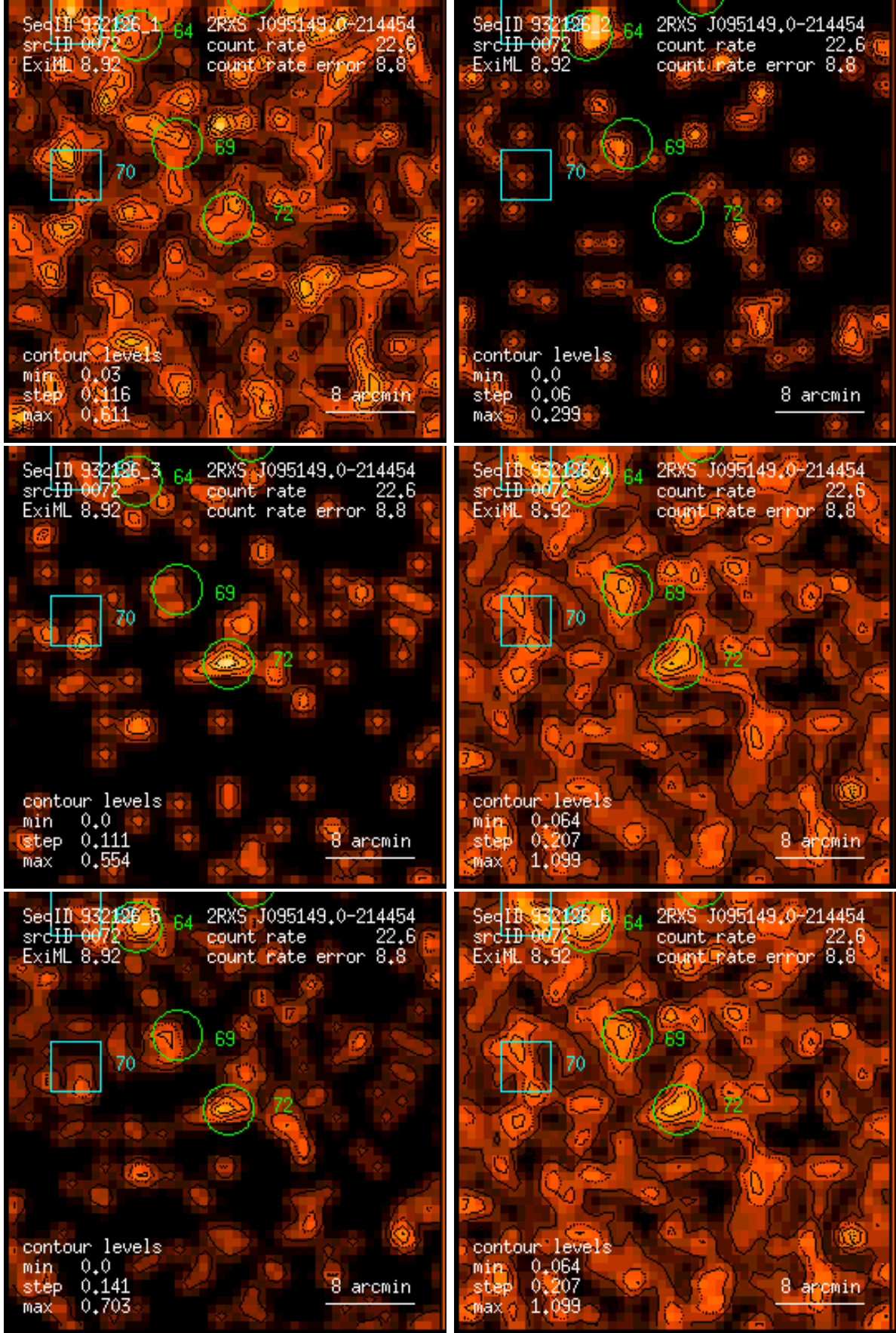
Figure 72: RASS 932126: detection 0072: band rate images, Gaussian filter: (1) PSPC channels 11 – 41, (2) 52 – 90, (3) 91 – 201, (4) 11 – 235, (5) 52 – 201, (6) 11 – 201. Broad band rates in counts/ks. Band rate contour levels in counts/ks/arcmin 2 .
