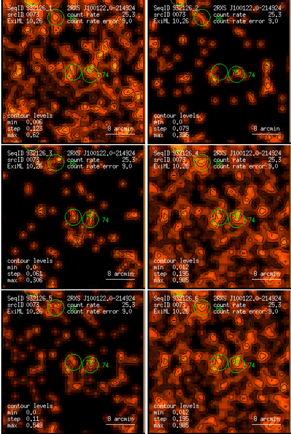
Figure 73: RASS 932126: detection 0073: band rate images, Gaussian filter: (1) PSPC channels 11 – 41, (2) 52 – 90, (3) 91 – 201, (4) 11 – 235, (5) 52 – 201, (6) 11 – 201. Broad band rates in counts/ks. Band rate contour levels in counts/ks/arcmin 2 .
