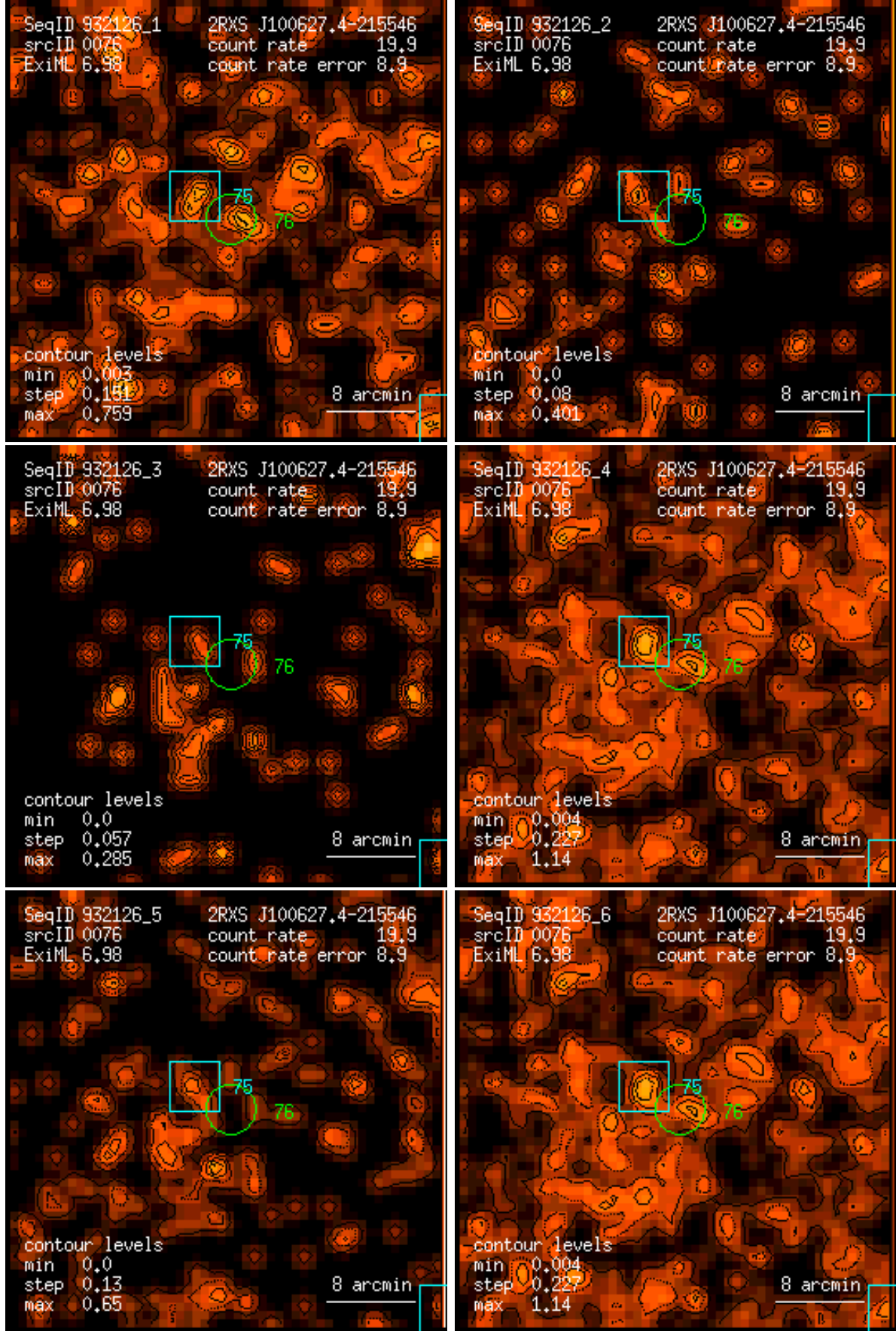
Figure 76: RASS 932126: detection 0076: band rate images, Gaussian filter: (1) PSPC channels 11 – 41, (2) 52 – 90, (3) 91 – 201, (4) 11 – 235, (5) 52 – 201, (6) 11 – 201. Broad band rates in counts/ks. Band rate contour levels in counts/ks/arcmin 2 .
