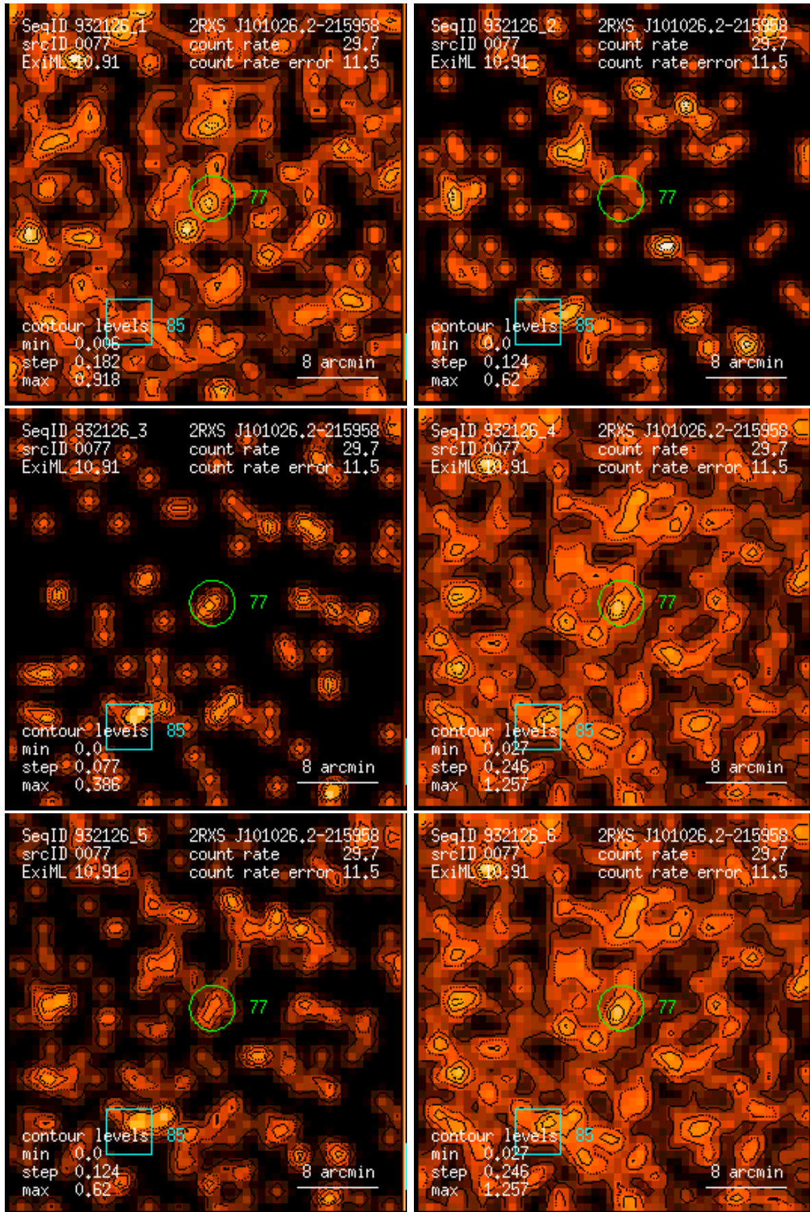
Figure 77: RASS 932126: detection 0077: band rate images, Gaussian filter: (1) PSPC channels 11 – 41, (2) 52 – 90, (3) 91 – 201, (4) 11 – 235, (5) 52 – 201, (6) 11 – 201. Broad band rates in counts/ks. Band rate contour levels in counts/ks/arcmin 2 .
