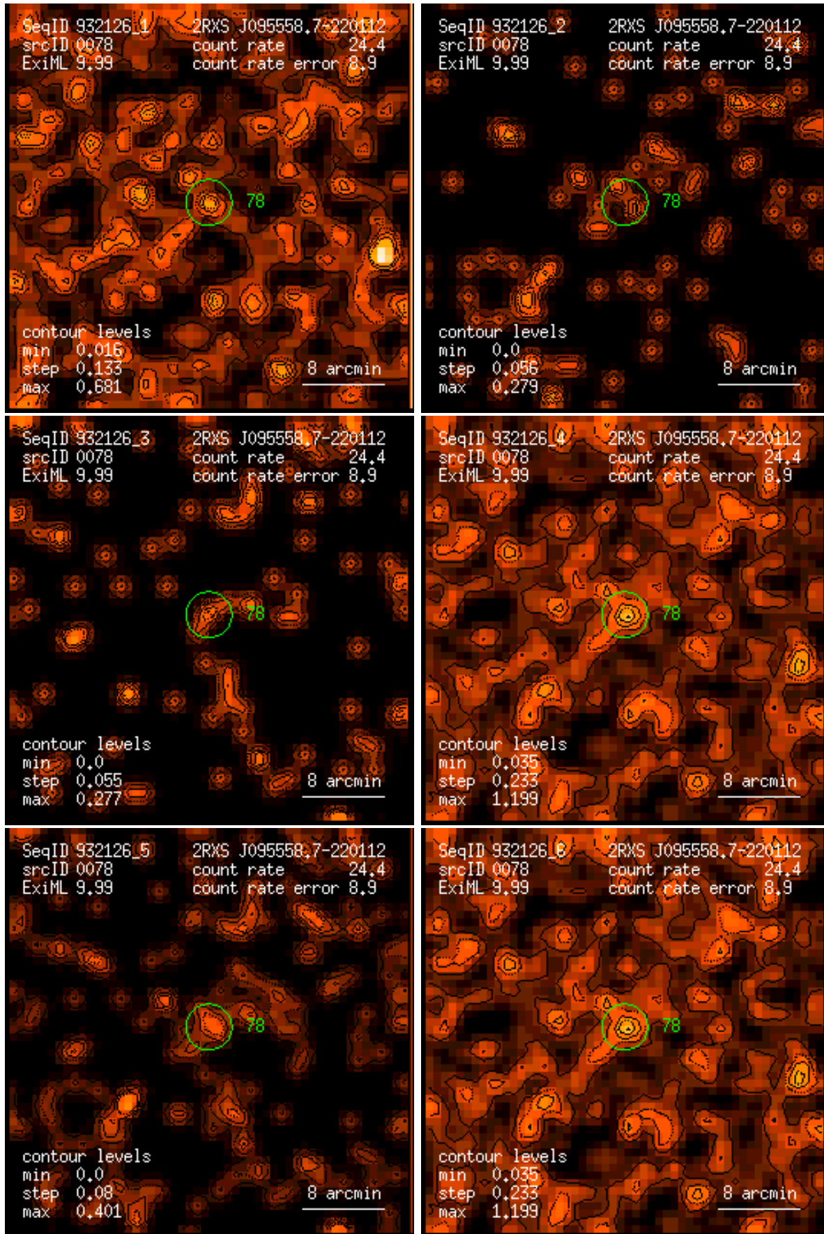
Figure 78: RASS 932126: detection 0078: band rate images, Gaussian filter: (1) PSPC channels 11 – 41, (2) 52 – 90, (3) 91 – 201, (4) 11 – 235, (5) 52 – 201, (6) 11 – 201. Broad band rates in counts/ks. Band rate contour levels in counts/ks/arcmin 2 .
