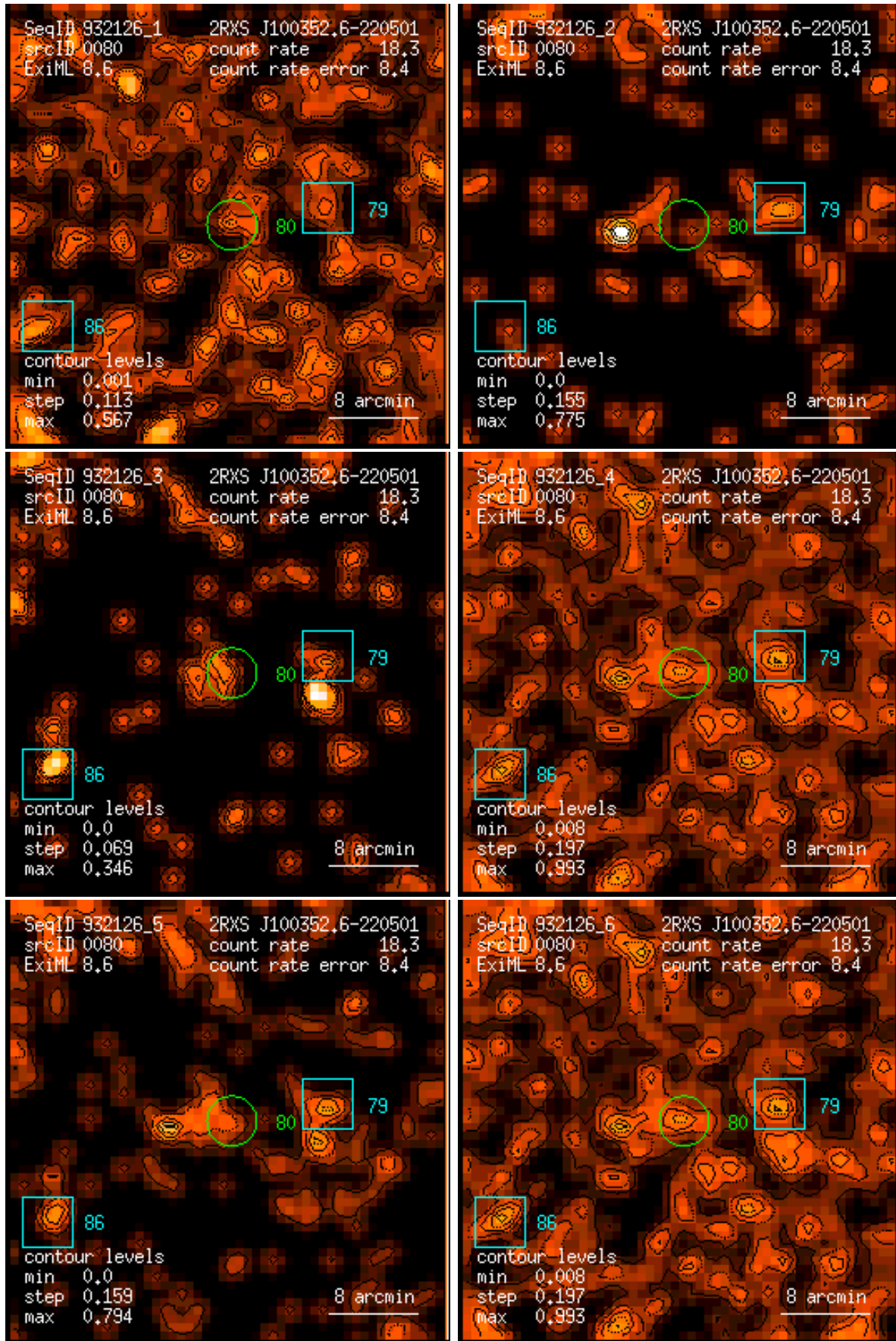
Figure 80: RASS 932126: detection 0080: band rate images, Gaussian filter: (1) PSPC channels 11 – 41, (2) 52 – 90, (3) 91 – 201, (4) 11 – 235, (5) 52 – 201, (6) 11 – 201. Broad band rates in counts/ks. Band rate contour levels in counts/ks/arcmin 2 .
