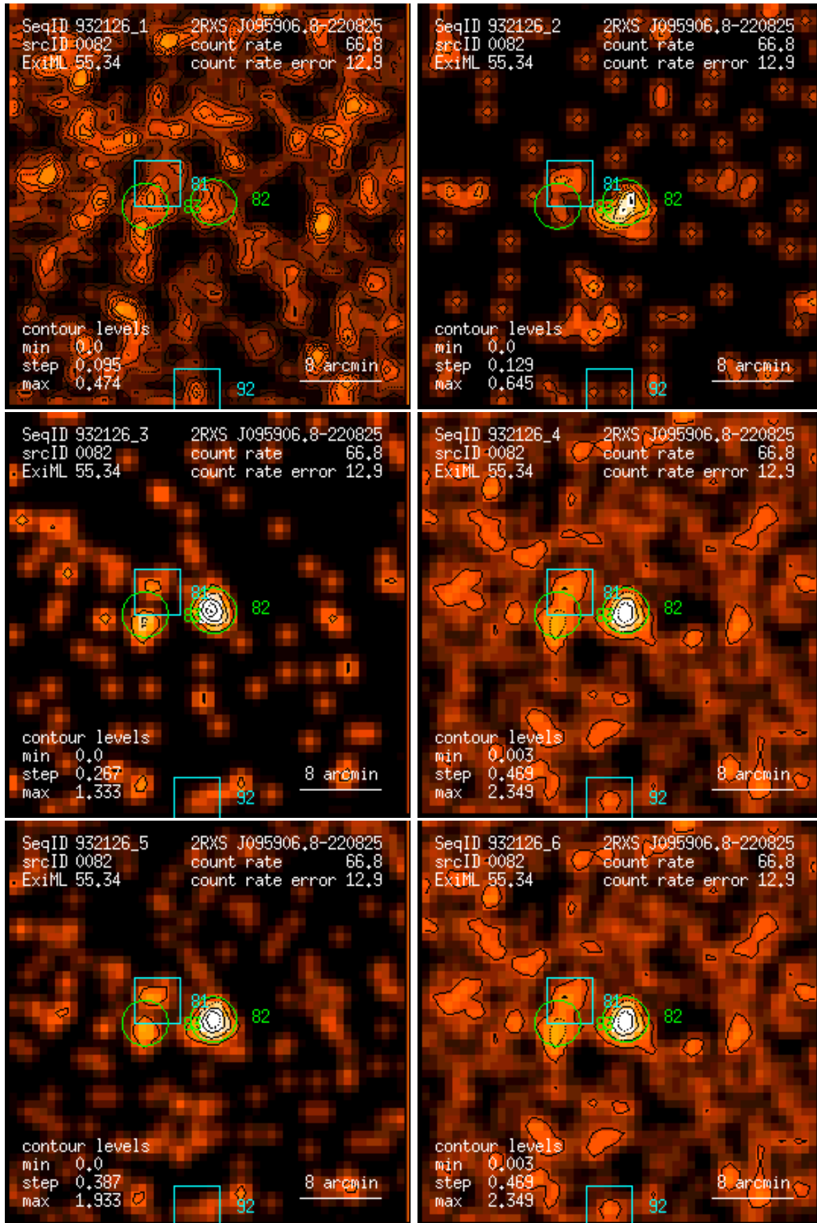
Figure 82: RASS 932126: detection 0082: band rate images, Gaussian filter: (1) PSPC channels 11 – 41, (2) 52 – 90, (3) 91 – 201, (4) 11 – 235, (5) 52 – 201, (6) 11 – 201. Broad band rates in counts/ks. Band rate contour levels in counts/ks/arcmin 2 .
