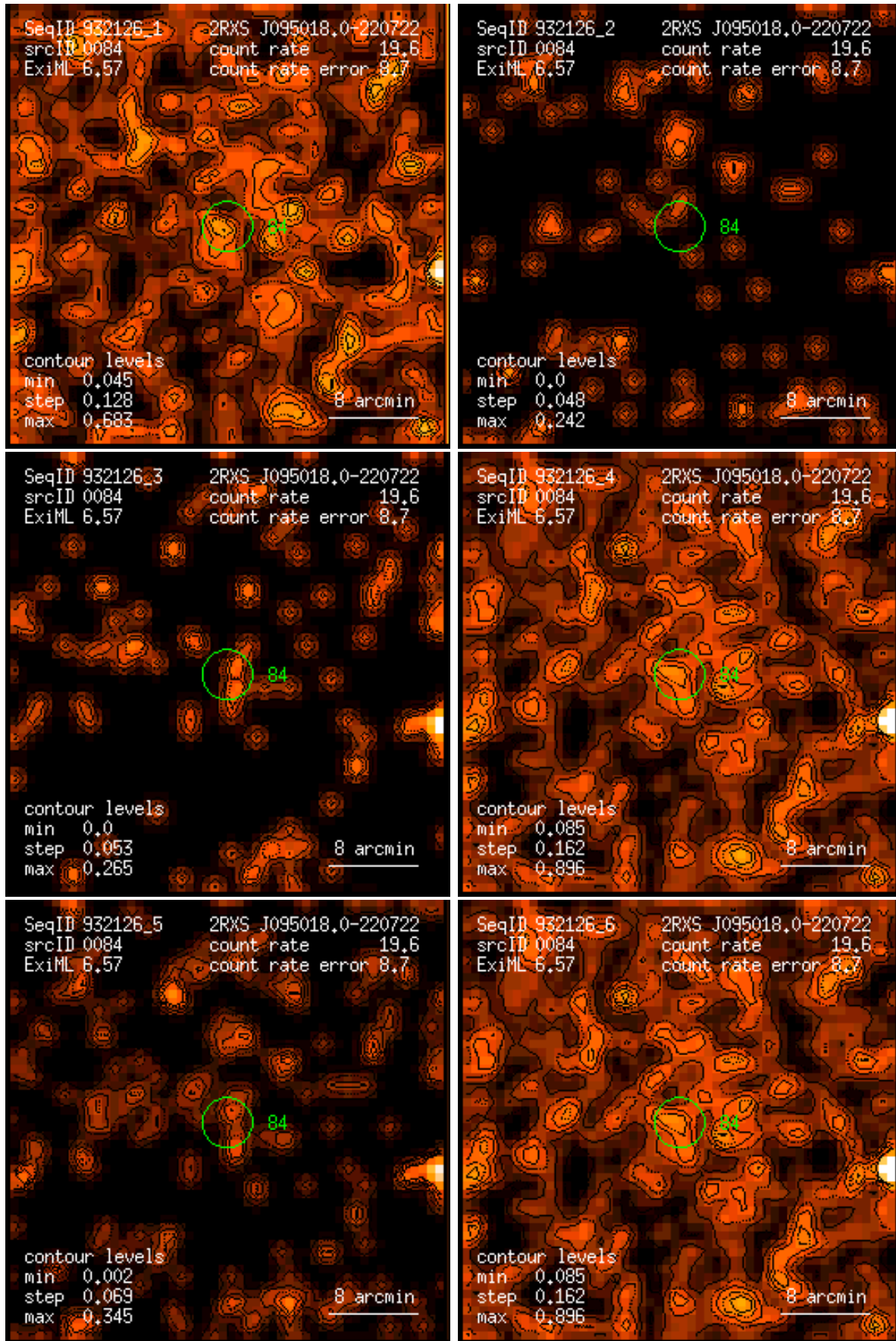
Figure 84: RASS 932126: detection 0084: band rate images, Gaussian filter: (1) PSPC channels 11 – 41, (2) 52 – 90, (3) 91 – 201, (4) 11 – 235, (5) 52 – 201, (6) 11 – 201. Broad band rates in counts/ks. Band rate contour levels in counts/ks/arcmin 2 .
