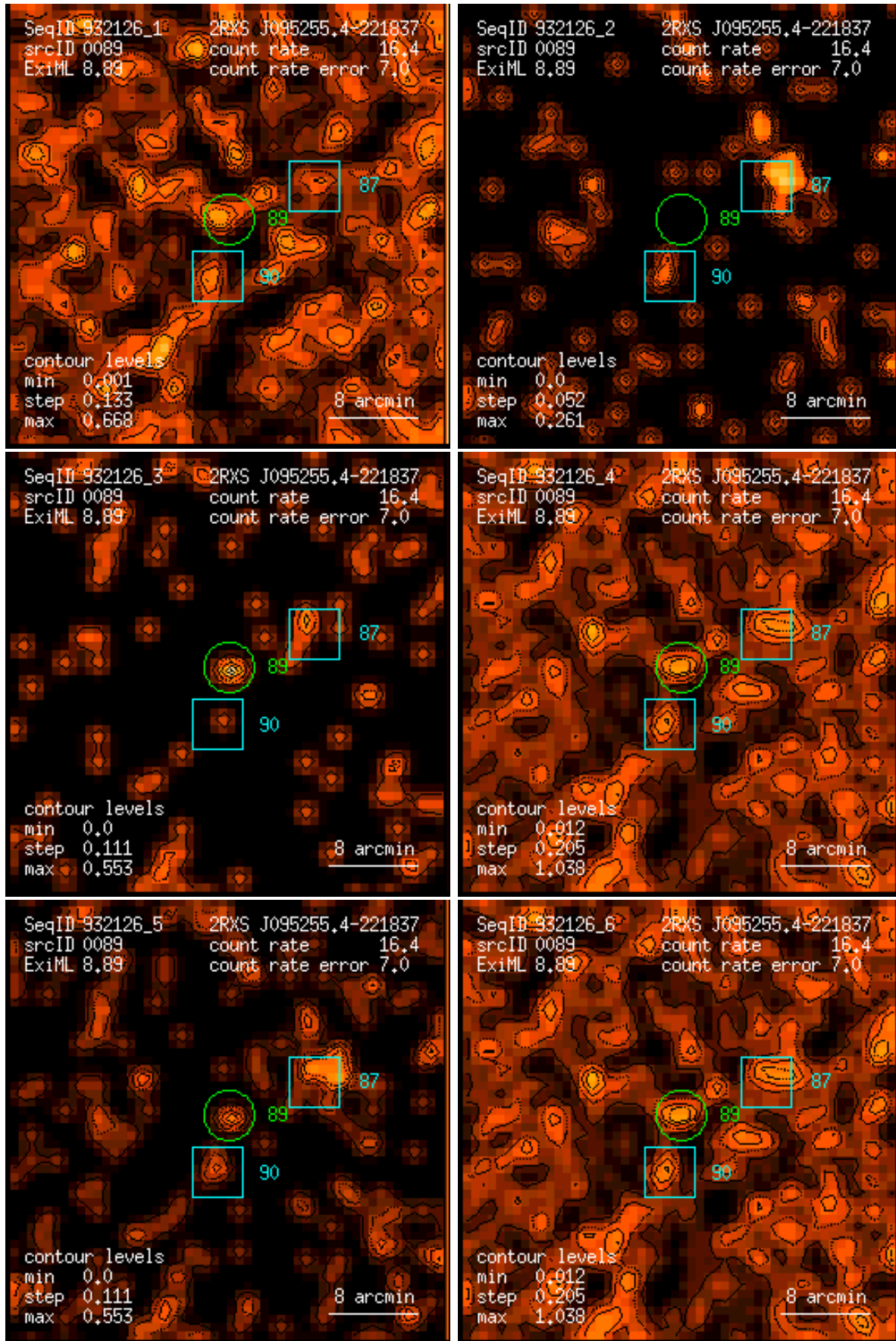
Figure 89: RASS 932126: detection 0089: band rate images, Gaussian filter: (1) PSPC channels 11 – 41, (2) 52 – 90, (3) 91 – 201, (4) 11 – 235, (5) 52 – 201, (6) 11 – 201. Broad band rates in counts/ks. Band rate contour levels in counts/ks/arcmin 2 .
