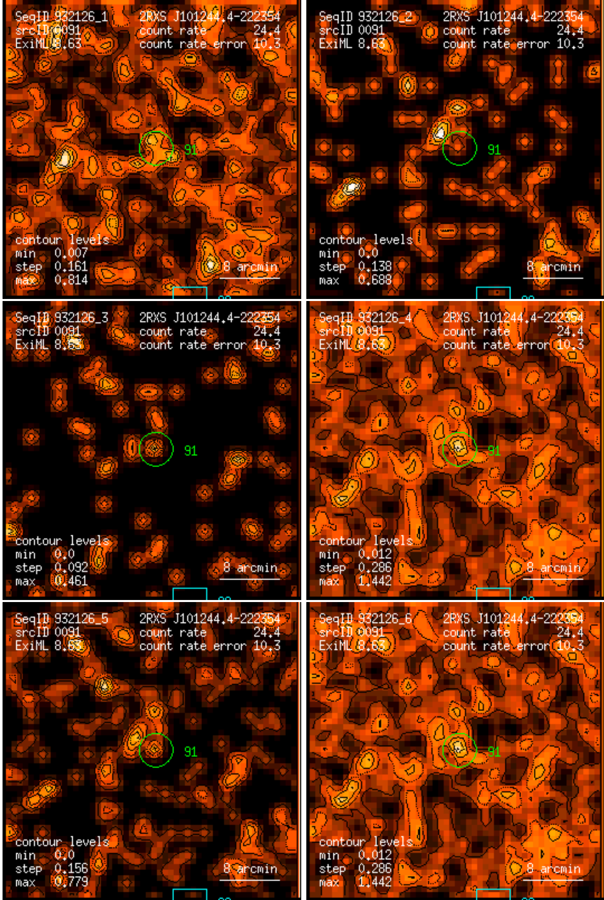
Figure 91: RASS 932126: detection 0091: band rate images, Gaussian filter: (1) PSPC channels 11 – 41, (2) 52 – 90, (3) 91 – 201, (4) 11 – 235, (5) 52 – 201, (6) 11 – 201. Broad band rates in counts/ks. Band rate contour levels in counts/ks/arcmin 2 .
