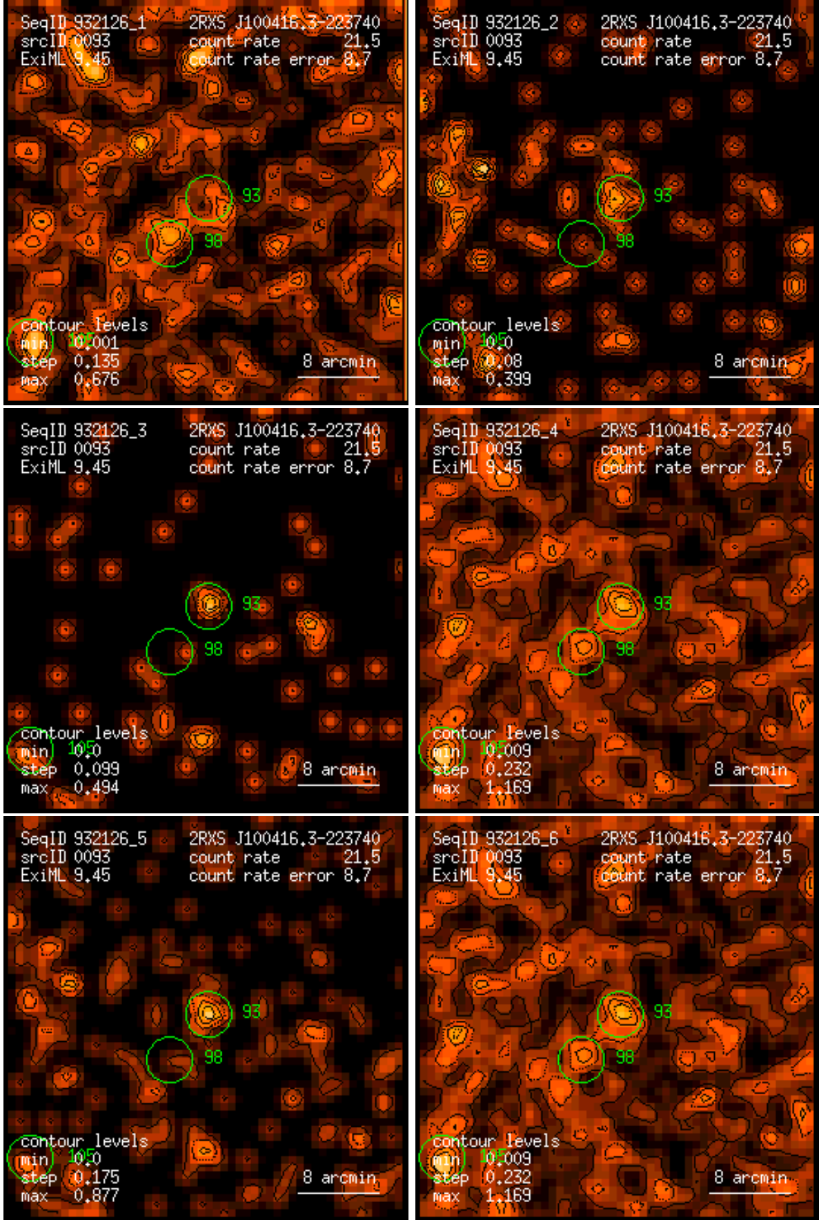
Figure 93: RASS 932126: detection 0093: band rate images, Gaussian filter: (1) PSPC channels 11 – 41, (2) 52 – 90, (3) 91 – 201, (4) 11 – 235, (5) 52 – 201, (6) 11 – 201. Broad band rates in counts/ks. Band rate contour levels in counts/ks/arcmin 2 .
