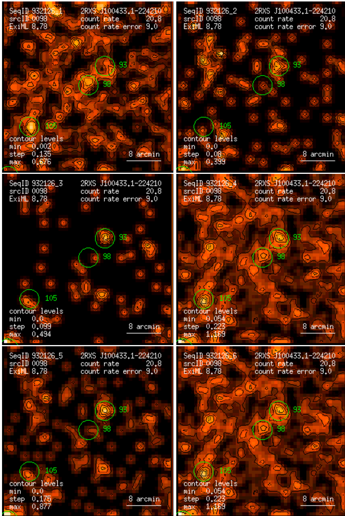
Figure 98: RASS 932126: detection 0098: band rate images, Gaussian filter: (1) PSPC channels 11 – 41, (2) 52 – 90, (3) 91 – 201, (4) 11 – 235, (5) 52 – 201, (6) 11 – 201. Broad band rates in counts/ks. Band rate contour levels in counts/ks/arcmin 2 .
