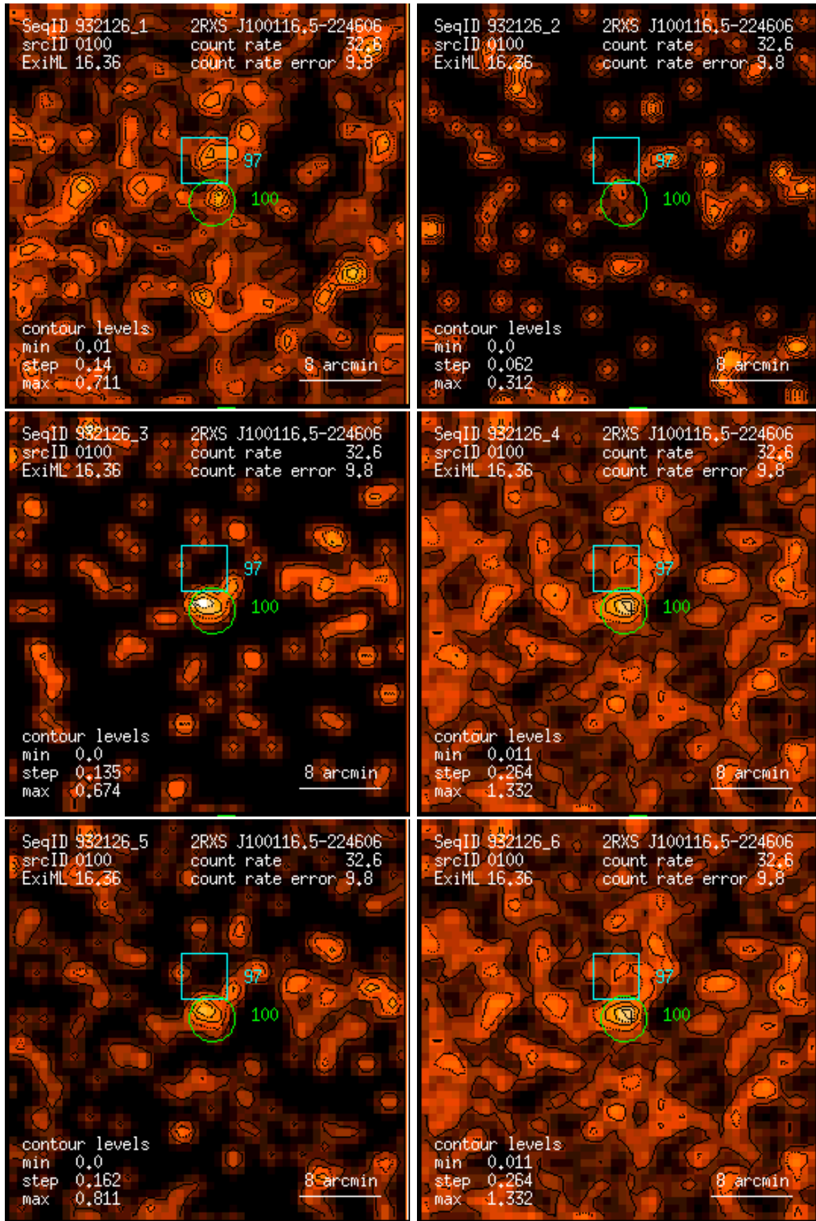
Figure 100: RASS 932126: detection 0100: band rate images, Gaussian filter: (1) PSPC channels 11 – 41, (2) 52 – 90, (3) 91 – 201, (4) 11 – 235, (5) 52 – 201, (6) 11 – 201. Broad band rates in counts/ks. Band rate contour levels in counts/ks/arcmin 2 .
