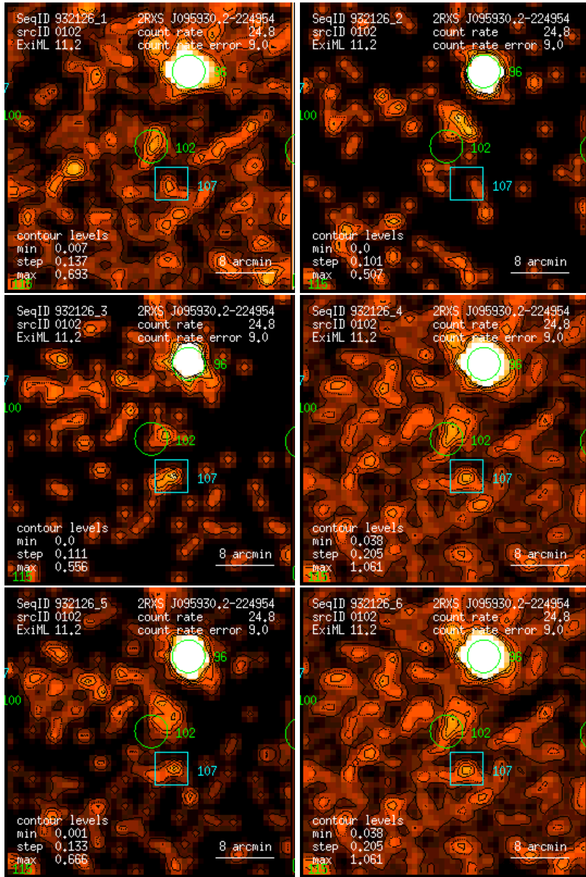
Figure 102: RASS 932126: detection 0102: band rate images, Gaussian filter: (1) PSPC channels 11 – 41, (2) 52 – 90, (3) 91 – 201, (4) 11 – 235, (5) 52 – 201, (6) 11 – 201. Broad band rates in counts/ks. Band rate contour levels in counts/ks/arcmin 2 .
