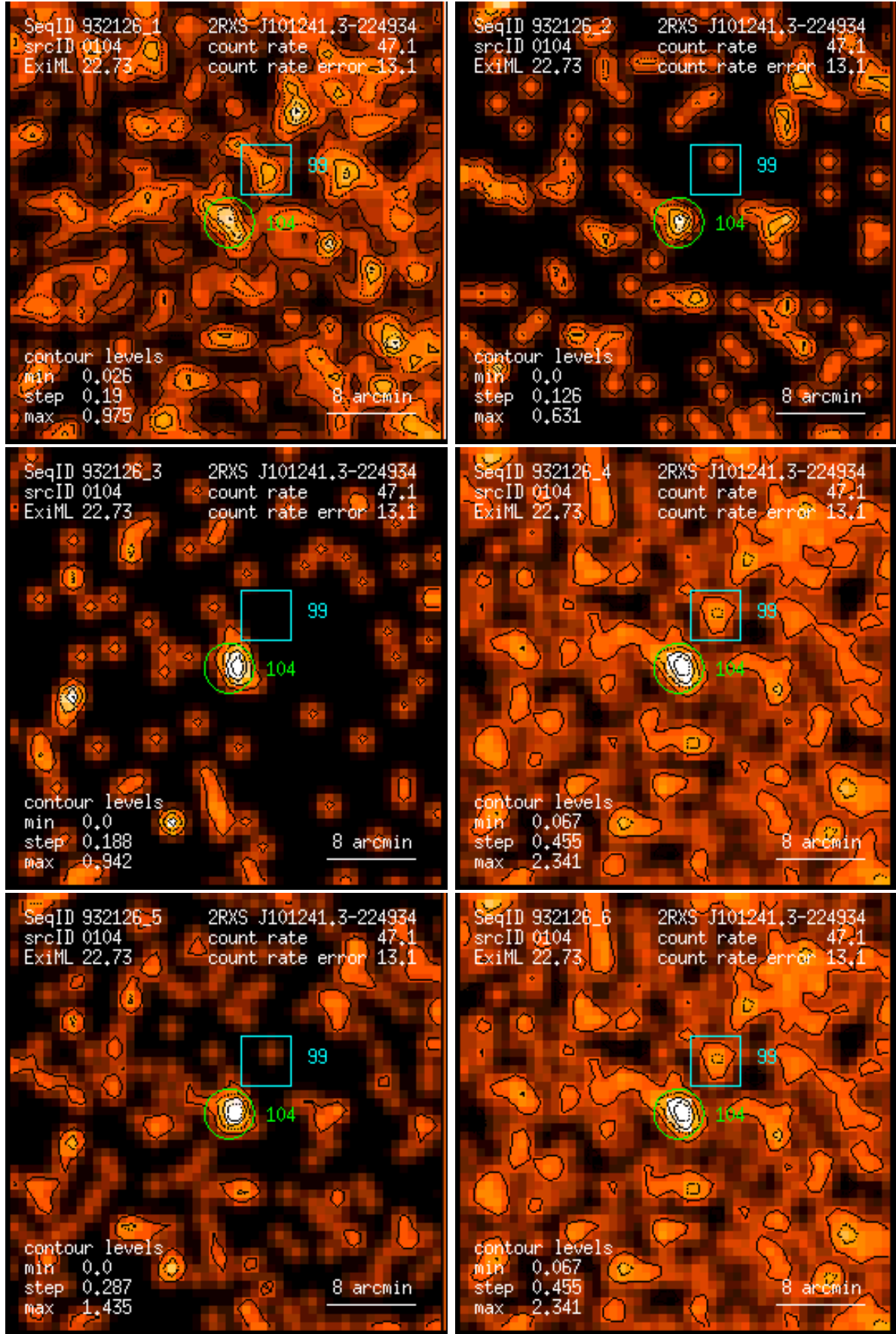
Figure 104: RASS 932126: detection 0104: band rate images, Gaussian filter: (1) PSPC channels 11 – 41, (2) 52 – 90, (3) 91 – 201, (4) 11 – 235, (5) 52 – 201, (6) 11 – 201. Broad band rates in counts/ks. Band rate contour levels in counts/ks/arcmin 2 .
