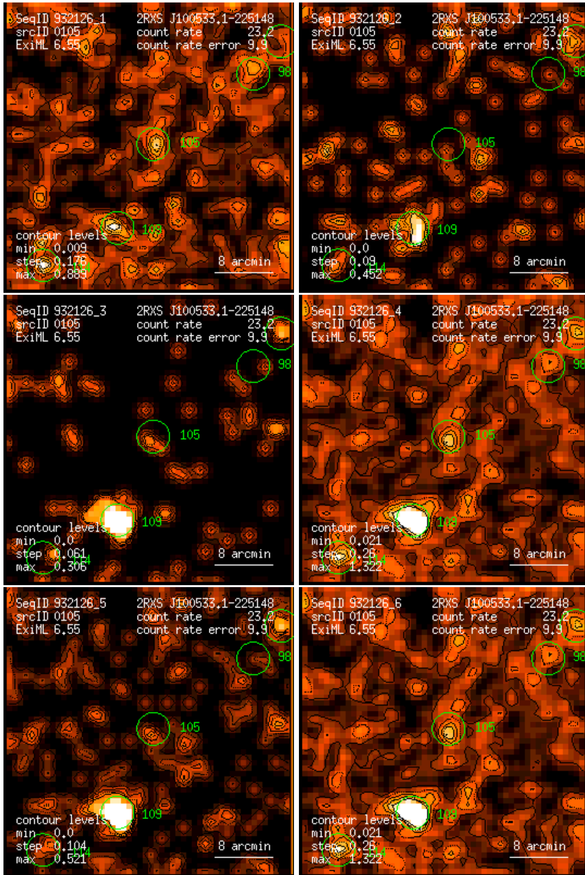
Figure 105: RASS 932126: detection 0105: band rate images, Gaussian filter: (1) PSPC channels 11 – 41, (2) 52 – 90, (3) 91 – 201, (4) 11 – 235, (5) 52 – 201, (6) 11 – 201. Broad band rates in counts/ks. Band rate contour levels in counts/ks/arcmin 2 .
