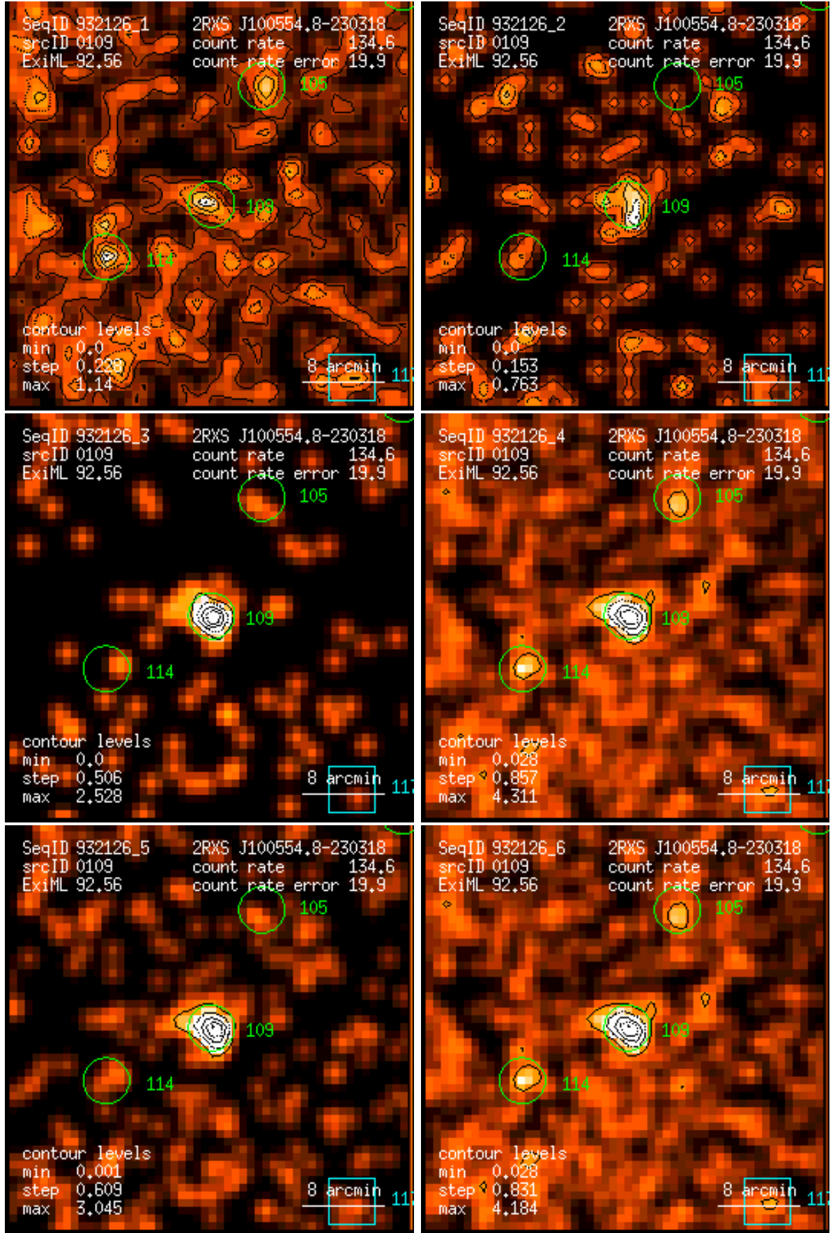
Figure 109: RASS 932126: detection 0109: band rate images, Gaussian filter: (1) PSPC channels 11 – 41, (2) 52 – 90, (3) 91 – 201, (4) 11 – 235, (5) 52 – 201, (6) 11 – 201. Broad band rates in counts/ks. Band rate contour levels in counts/ks/arcmin 2 .
