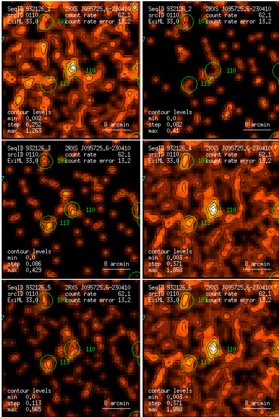
Figure 110: RASS 932126: detection 0110: band rate images, Gaussian filter: (1) PSPC channels 11 – 41, (2) 52 – 90, (3) 91 – 201, (4) 11 – 235, (5) 52 – 201, (6) 11 – 201. Broad band rates in counts/ks. Band rate contour levels in counts/ks/arcmin 2 .
