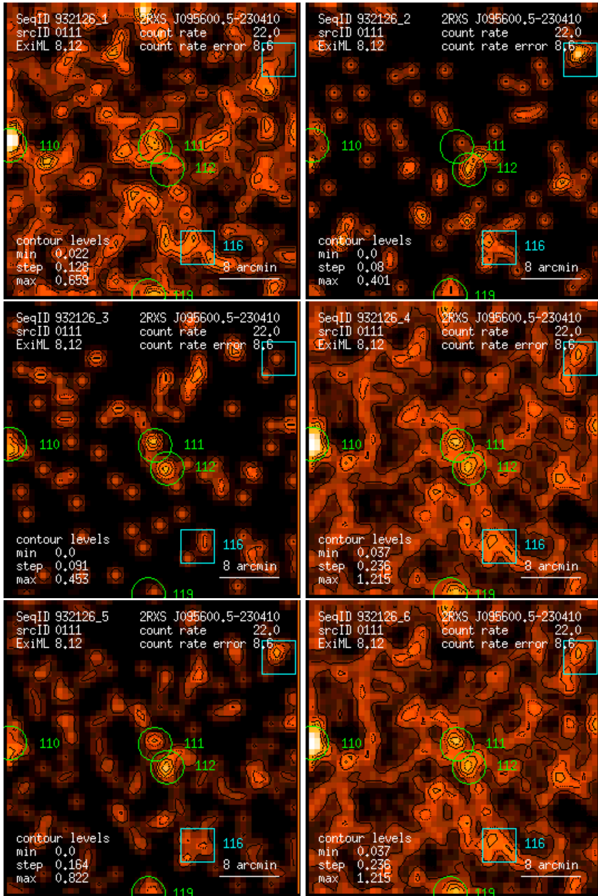
Figure 111: RASS 932126: detection 0111: band rate images, Gaussian filter: (1) PSPC channels 11 – 41, (2) 52 – 90, (3) 91 – 201, (4) 11 – 235, (5) 52 – 201, (6) 11 – 201. Broad band rates in counts/ks. Band rate contour levels in counts/ks/arcmin 2 .
