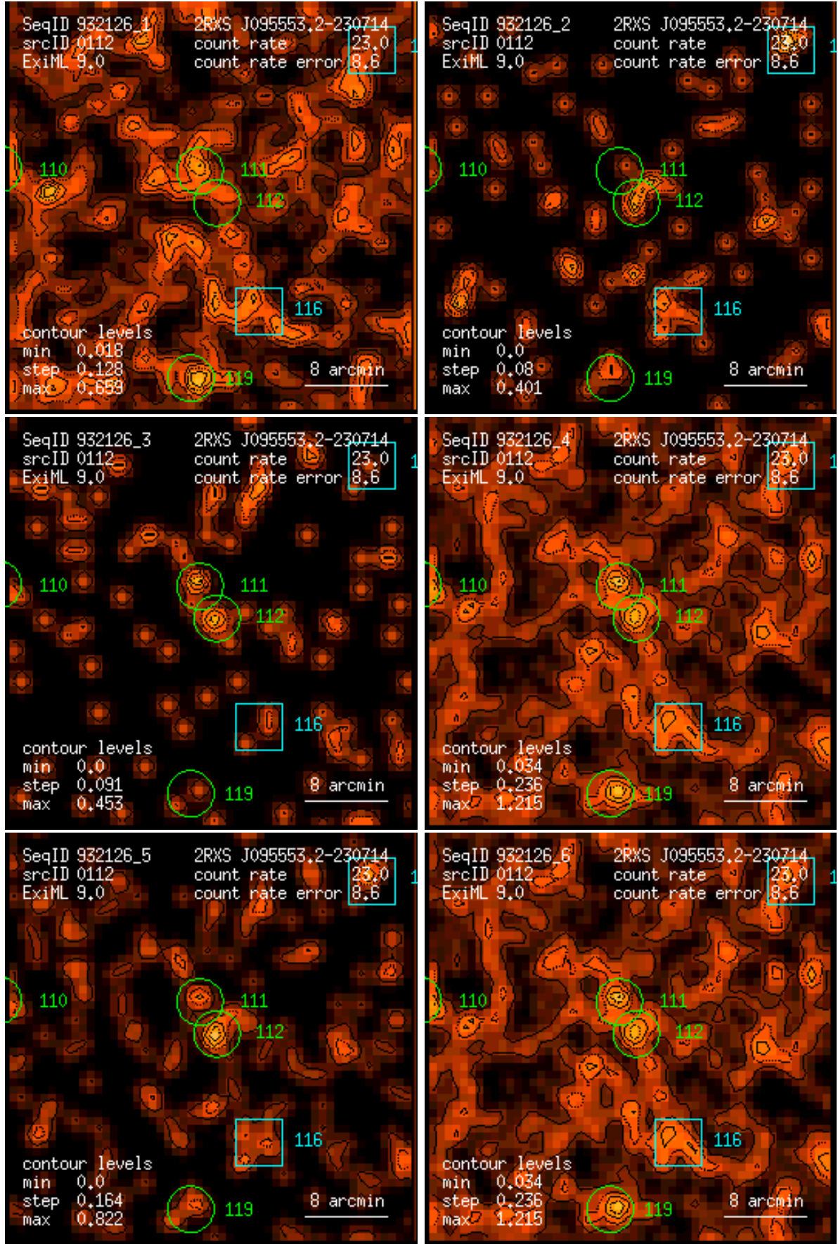
Figure 112: RASS 932126: detection 0112: band rate images, Gaussian filter: (1) PSPC channels 11 – 41, (2) 52 – 90, (3) 91 – 201, (4) 11 – 235, (5) 52 – 201, (6) 11 – 201. Broad band rates in counts/ks. Band rate contour levels in counts/ks/arcmin 2 .
