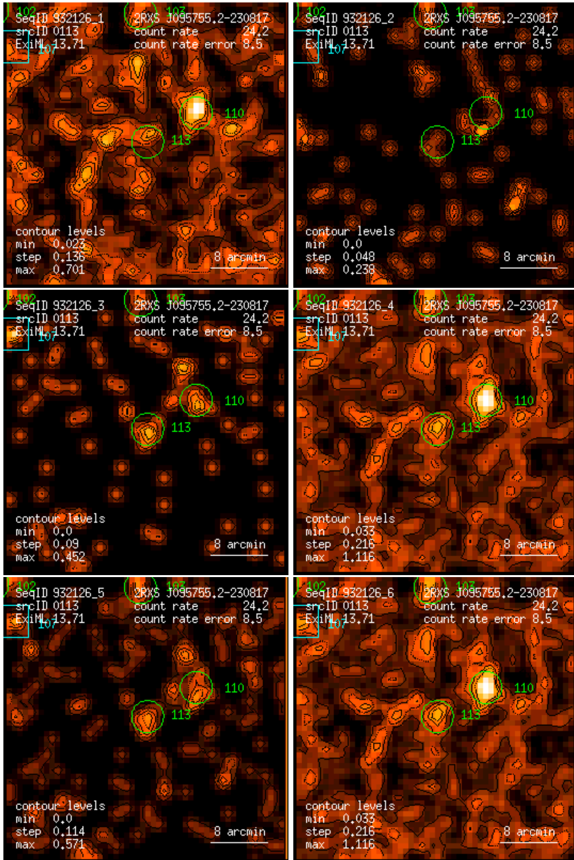
Figure 113: RASS 932126: detection 0113: band rate images, Gaussian filter: (1) PSPC channels 11 – 41, (2) 52 – 90, (3) 91 – 201, (4) 11 – 235, (5) 52 – 201, (6) 11 – 201. Broad band rates in counts/ks. Band rate contour levels in counts/ks/arcmin 2 .
