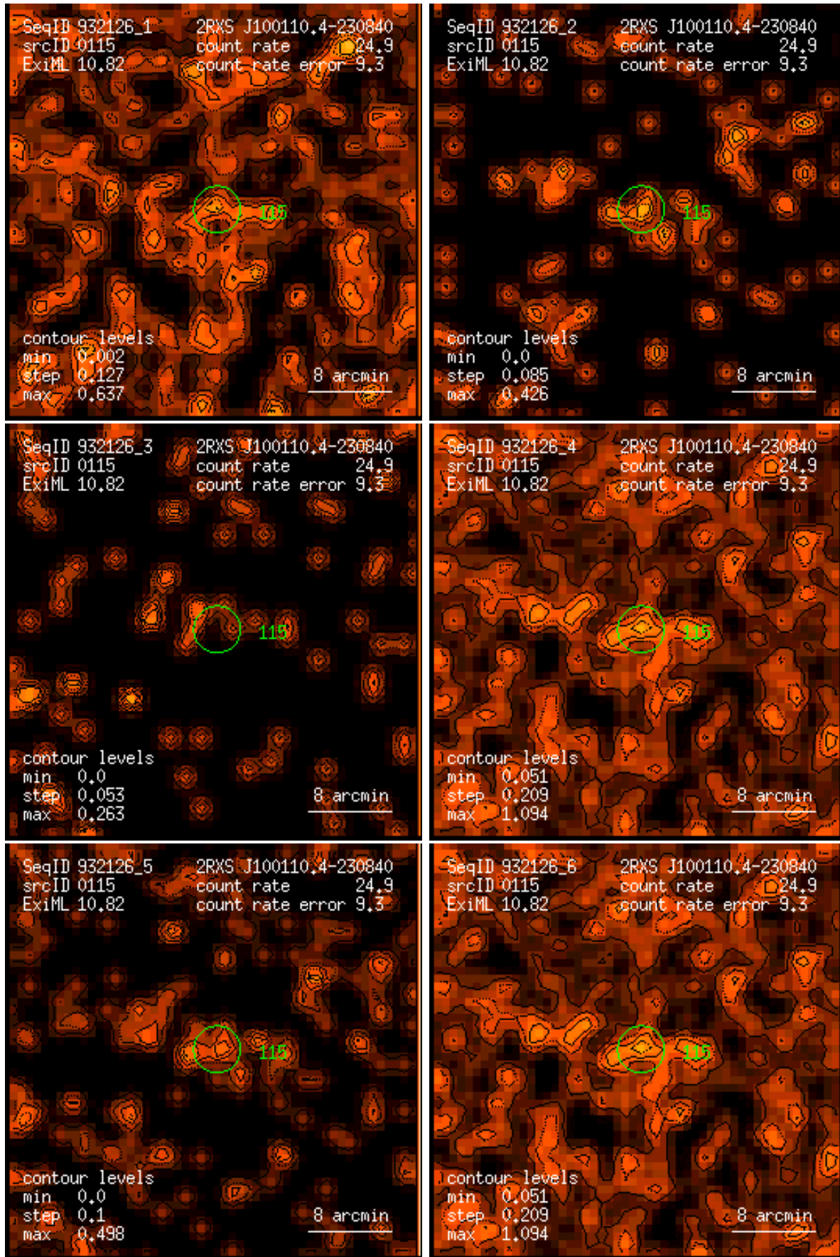
Figure 115: RASS 932126: detection 0115: band rate images, Gaussian filter: (1) PSPC channels 11 – 41, (2) 52 – 90, (3) 91 – 201, (4) 11 – 235, (5) 52 – 201, (6) 11 – 201. Broad band rates in counts/ks. Band rate contour levels in counts/ks/arcmin 2 .
