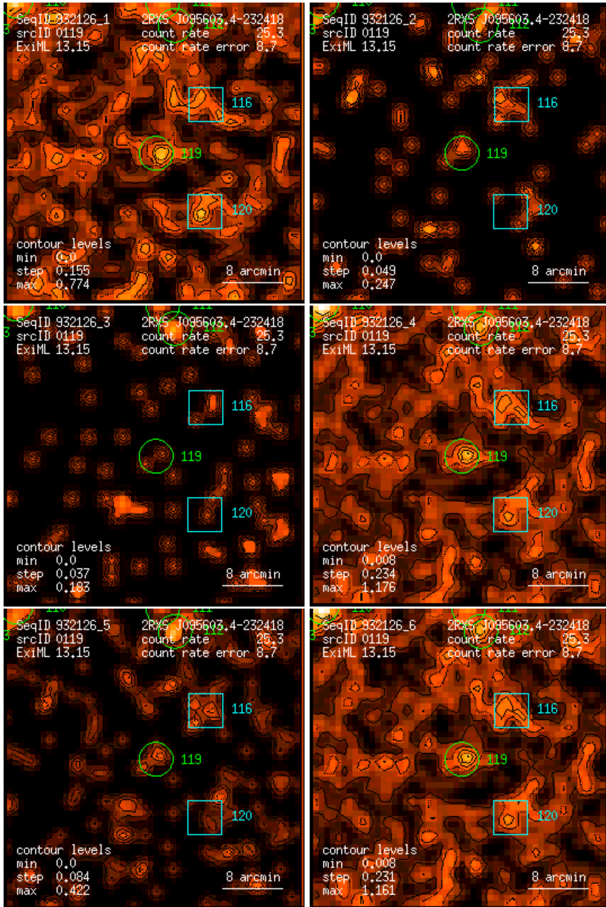
Figure 119: RASS 932126: detection 0119: band rate images, Gaussian filter: (1) PSPC channels 11 – 41, (2) 52 – 90, (3) 91 – 201, (4) 11 – 235, (5) 52 – 201, (6) 11 – 201. Broad band rates in counts/ks. Band rate contour levels in counts/ks/arcmin 2 .
