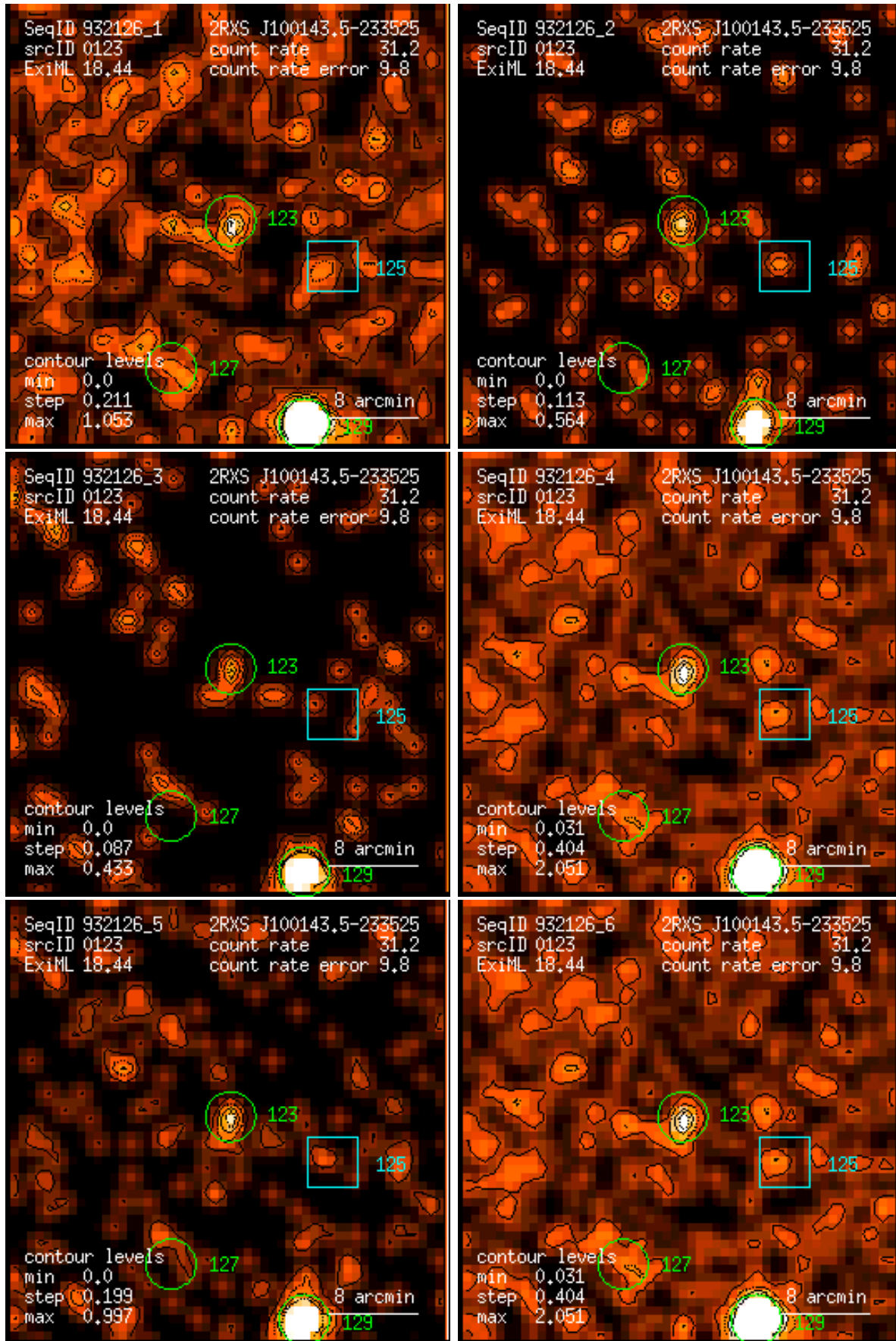
Figure 123: RASS 932126: detection 0123: band rate images, Gaussian filter: (1) PSPC channels 11 – 41, (2) 52 – 90, (3) 91 – 201, (4) 11 – 235, (5) 52 – 201, (6) 11 – 201. Broad band rates in counts/ks. Band rate contour levels in counts/ks/arcmin 2 .
