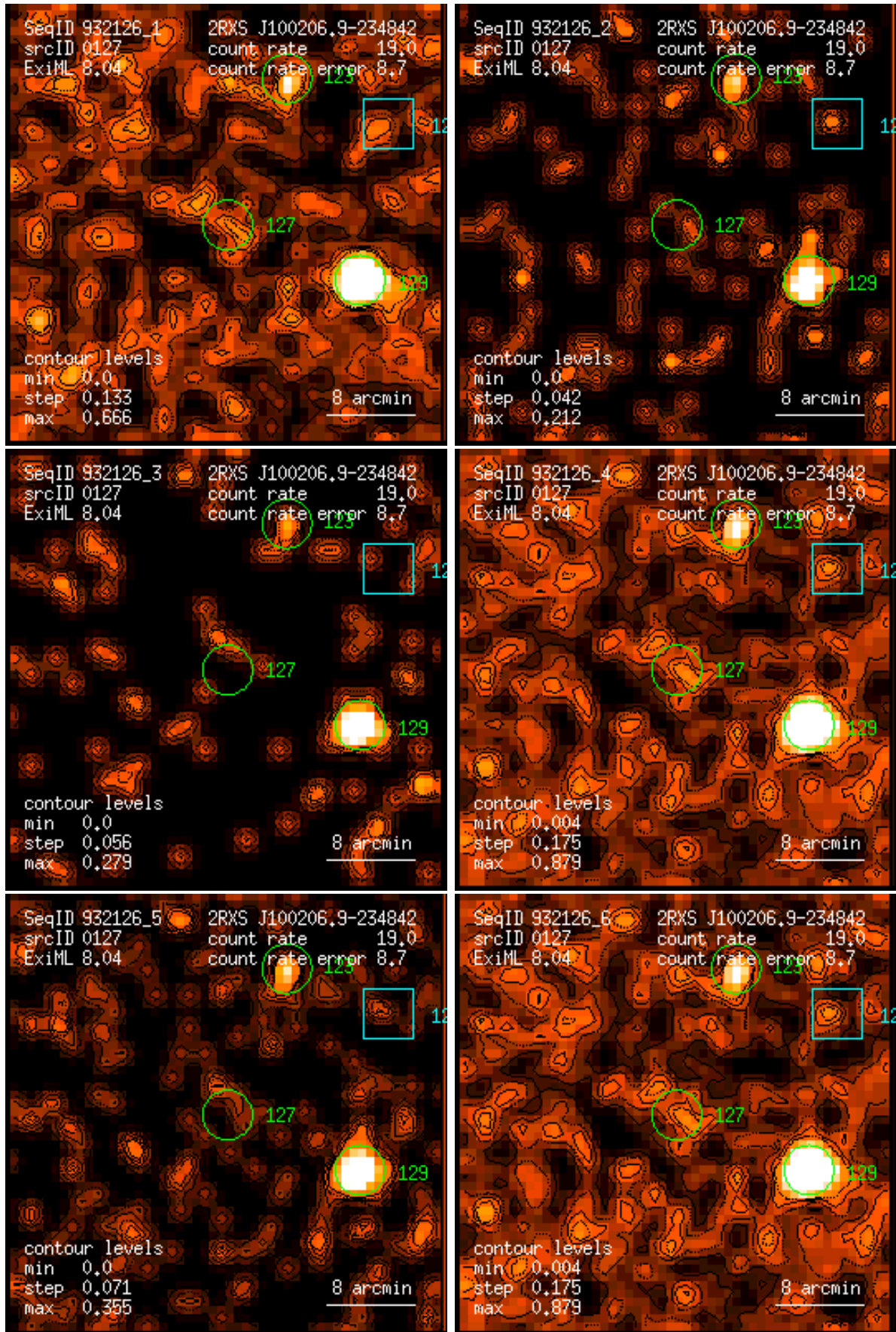
Figure 127: RASS 932126: detection 0127: band rate images, Gaussian filter: (1) PSPC channels 11 – 41, (2) 52 – 90, (3) 91 – 201, (4) 11 – 235, (5) 52 – 201, (6) 11 – 201. Broad band rates in counts/ks. Band rate contour levels in counts/ks/arcmin 2 .
