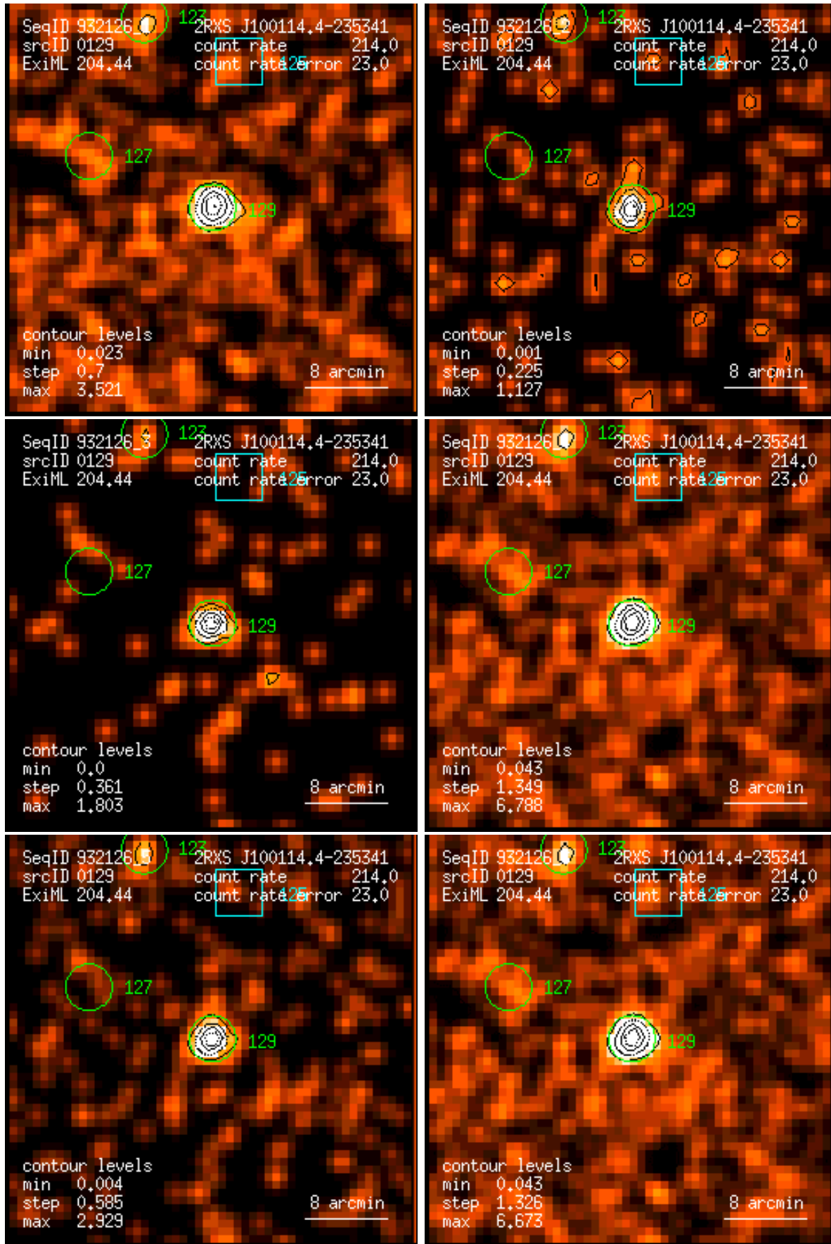
Figure 129: RASS 932126: detection 0129: band rate images, Gaussian filter: (1) PSPC channels 11 – 41, (2) 52 – 90, (3) 91 – 201, (4) 11 – 235, (5) 52 – 201, (6) 11 – 201. Broad band rates in counts/ks. Band rate contour levels in counts/ks/arcmin 2 .
