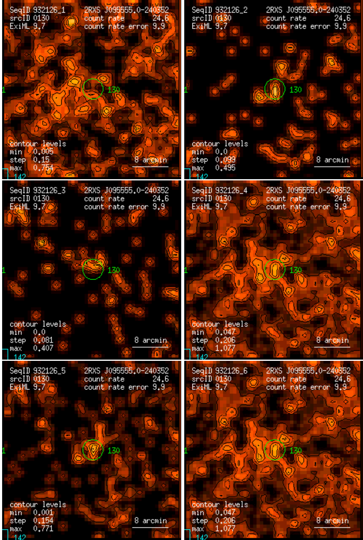
Figure 130: RASS 932126: detection 0130: band rate images, Gaussian filter: (1) PSPC channels 11 – 41, (2) 52 – 90, (3) 91 – 201, (4) 11 – 235, (5) 52 – 201, (6) 11 – 201. Broad band rates in counts/ks. Band rate contour levels in counts/ks/arcmin 2 .
