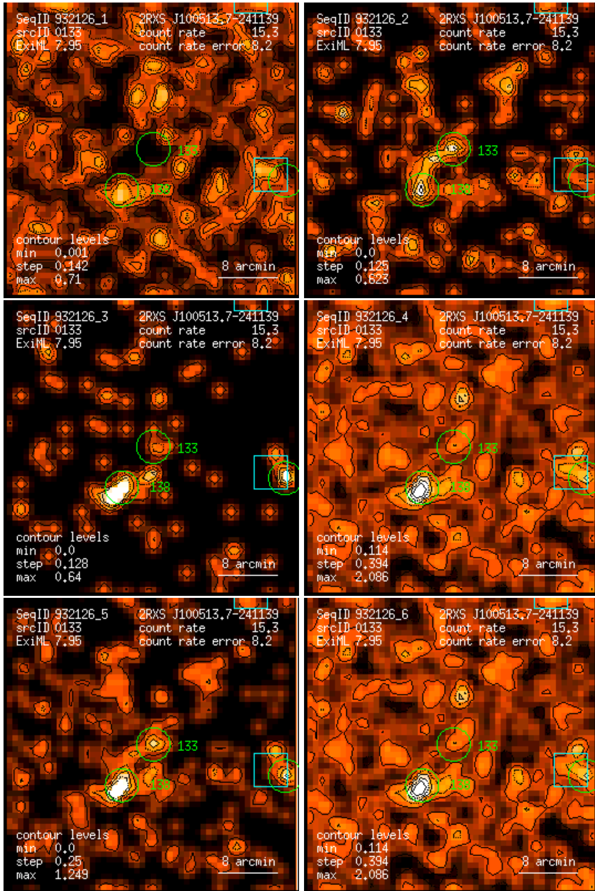
Figure 133: RASS 932126: detection 0133: band rate images, Gaussian filter: (1) PSPC channels 11 – 41, (2) 52 – 90, (3) 91 – 201, (4) 11 – 235, (5) 52 – 201, (6) 11 – 201. Broad band rates in counts/ks. Band rate contour levels in counts/ks/arcmin 2 .
