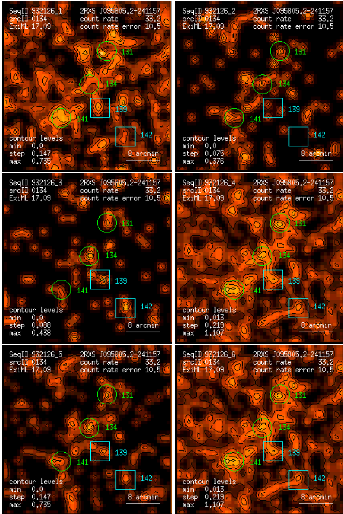
Figure 134: RASS 932126: detection 0134: band rate images, Gaussian filter: (1) PSPC channels 11 – 41, (2) 52 – 90, (3) 91 – 201, (4) 11 – 235, (5) 52 – 201, (6) 11 – 201. Broad band rates in counts/ks. Band rate contour levels in counts/ks/arcmin 2 .
