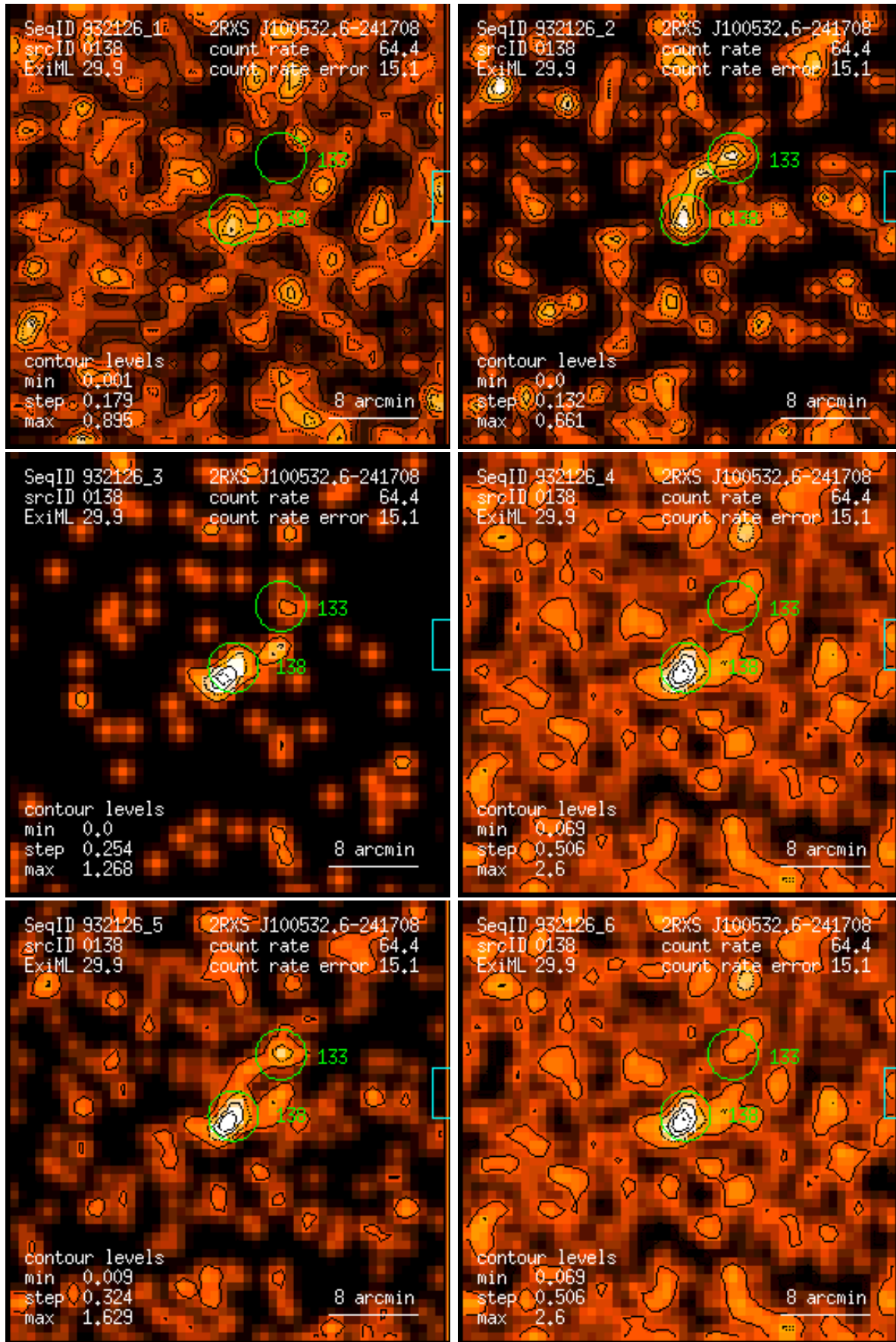
Figure 138: RASS 932126: detection 0138: band rate images, Gaussian filter: (1) PSPC channels 11 – 41, (2) 52 – 90, (3) 91 – 201, (4) 11 – 235, (5) 52 – 201, (6) 11 – 201. Broad band rates in counts/ks. Band rate contour levels in counts/ks/arcmin 2 .
