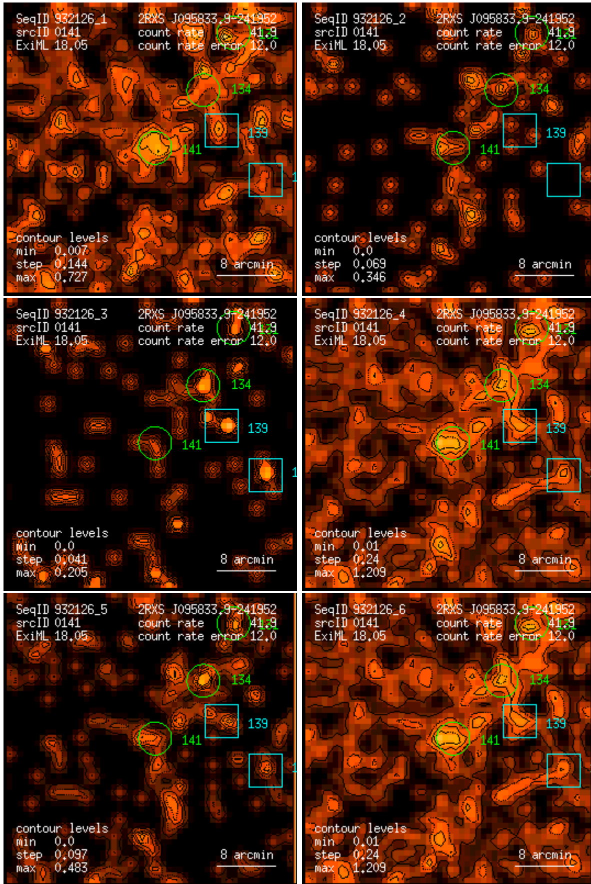
Figure 141: RASS 932126: detection 0141: band rate images, Gaussian filter: (1) PSPC channels 11 – 41, (2) 52 – 90, (3) 91 – 201, (4) 11 – 235, (5) 52 – 201, (6) 11 – 201. Broad band rates in counts/ks. Band rate contour levels in counts/ks/arcmin 2 .
