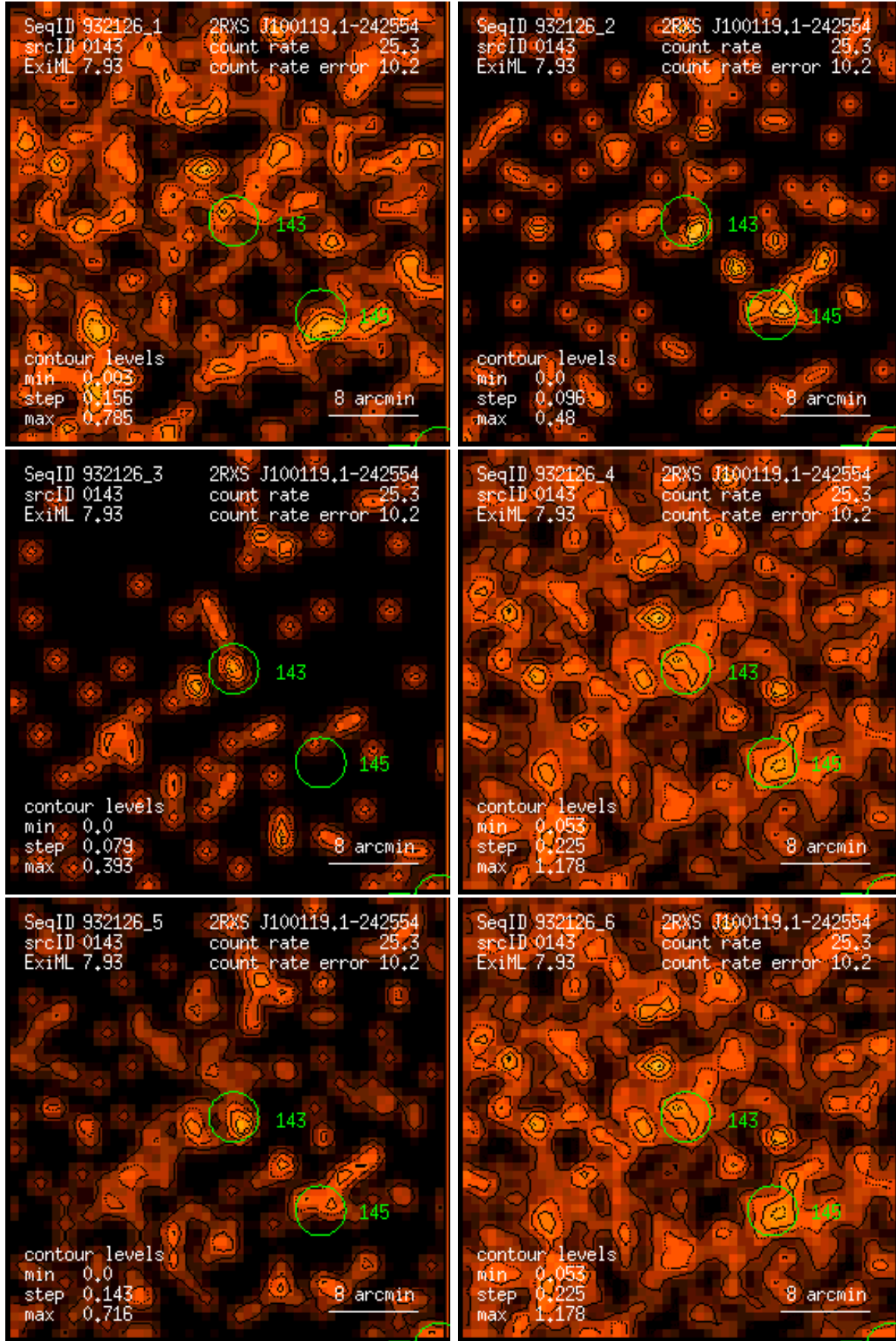
Figure 143: RASS 932126: detection 0143: band rate images, Gaussian filter: (1) PSPC channels 11 – 41, (2) 52 – 90, (3) 91 – 201, (4) 11 – 235, (5) 52 – 201, (6) 11 – 201. Broad band rates in counts/ks. Band rate contour levels in counts/ks/arcmin 2 .
