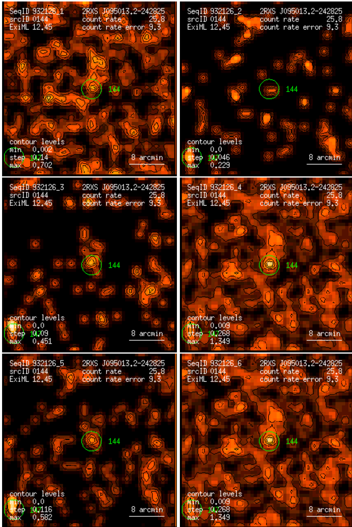
Figure 144: RASS 932126: detection 0144: band rate images, Gaussian filter: (1) PSPC channels 11 – 41, (2) 52 – 90, (3) 91 – 201, (4) 11 – 235, (5) 52 – 201, (6) 11 – 201. Broad band rates in counts/ks. Band rate contour levels in counts/ks/arcmin 2 .
