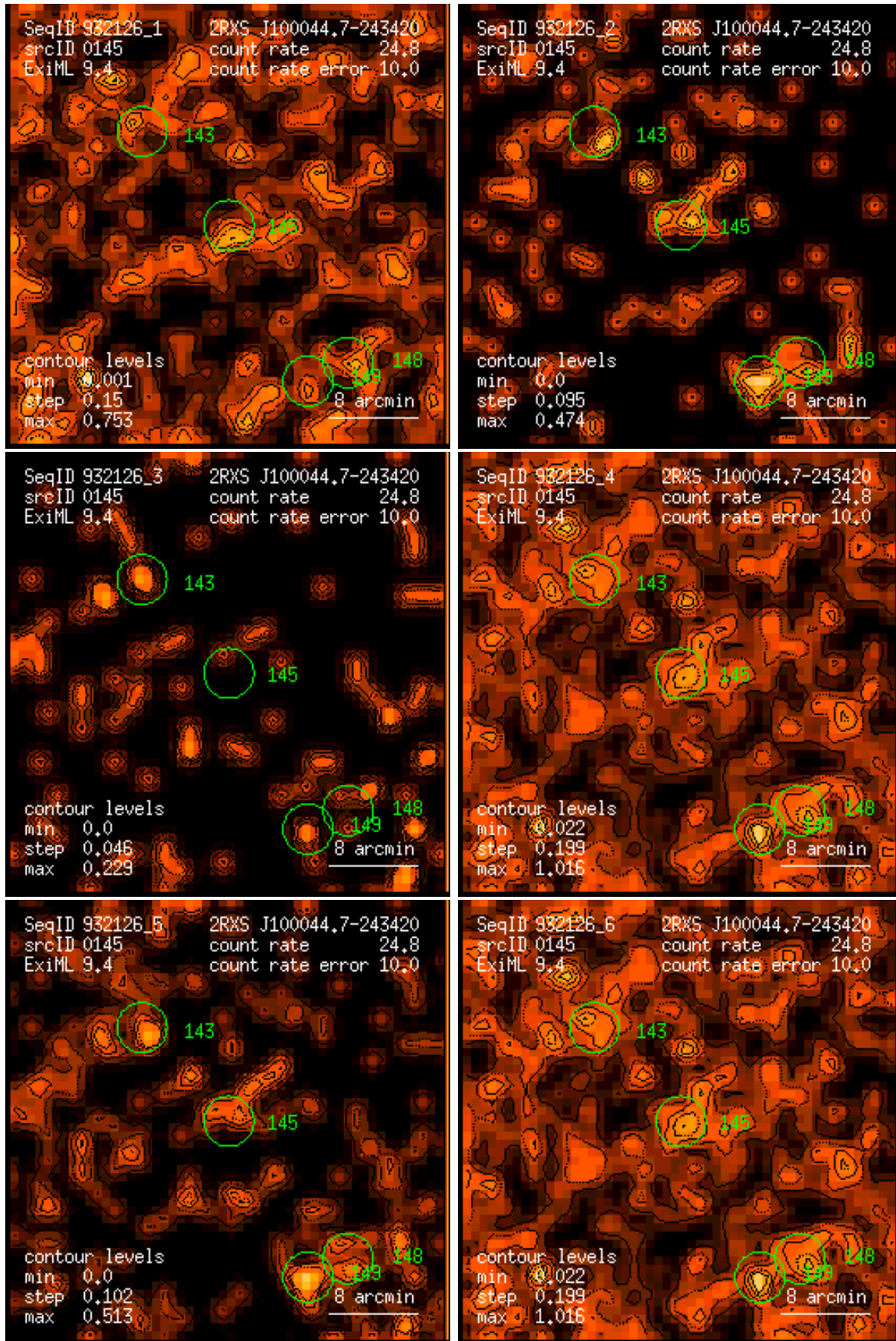
Figure 145: RASS 932126: detection 0145: band rate images, Gaussian filter: (1) PSPC channels 11 – 41, (2) 52 – 90, (3) 91 – 201, (4) 11 – 235, (5) 52 – 201, (6) 11 – 201. Broad band rates in counts/ks. Band rate contour levels in counts/ks/arcmin 2 .
