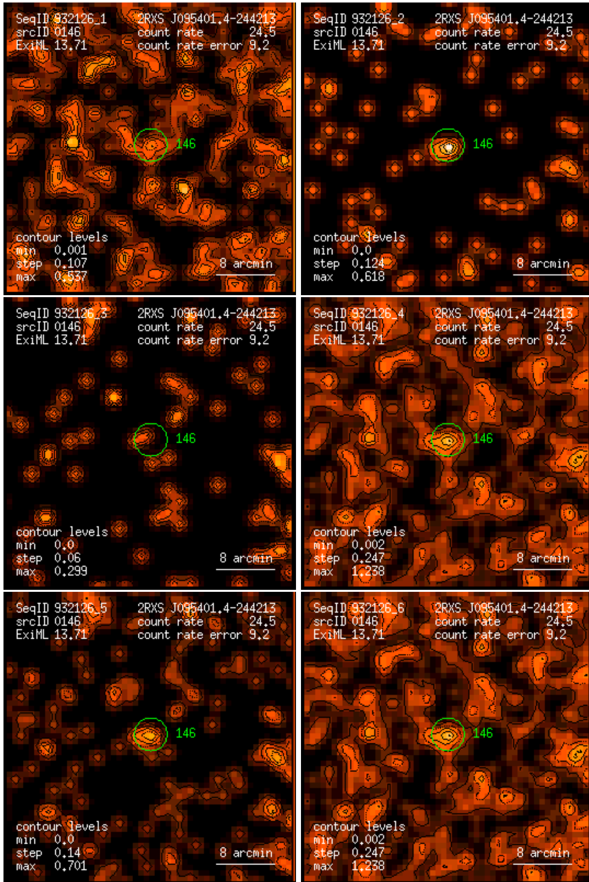
Figure 146: RASS 932126: detection 0146: band rate images, Gaussian filter: (1) PSPC channels 11 – 41, (2) 52 – 90, (3) 91 – 201, (4) 11 – 235, (5) 52 – 201, (6) 11 – 201. Broad band rates in counts/ks. Band rate contour levels in counts/ks/arcmin 2 .
