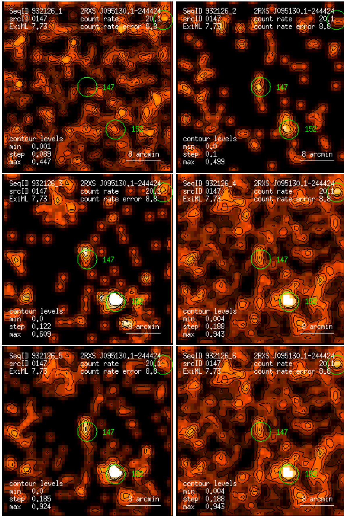
Figure 147: RASS 932126: detection 0147: band rate images, Gaussian filter: (1) PSPC channels 11 – 41, (2) 52 – 90, (3) 91 – 201, (4) 11 – 235, (5) 52 – 201, (6) 11 – 201. Broad band rates in counts/ks. Band rate contour levels in counts/ks/arcmin 2 .
