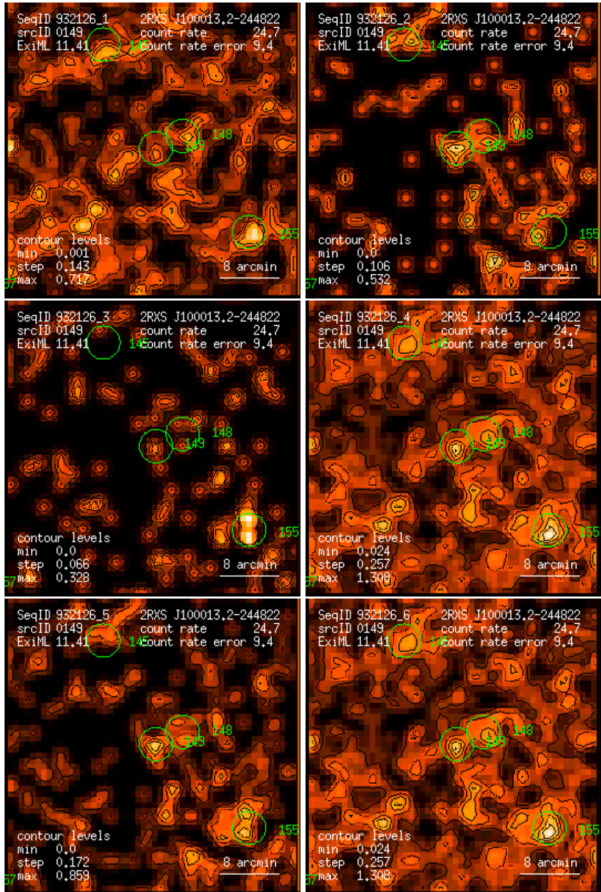
Figure 149: RASS 932126: detection 0149: band rate images, Gaussian filter: (1) PSPC channels 11 – 41, (2) 52 – 90, (3) 91 – 201, (4) 11 – 235, (5) 52 – 201, (6) 11 – 201. Broad band rates in counts/ks. Band rate contour levels in counts/ks/arcmin 2 .
