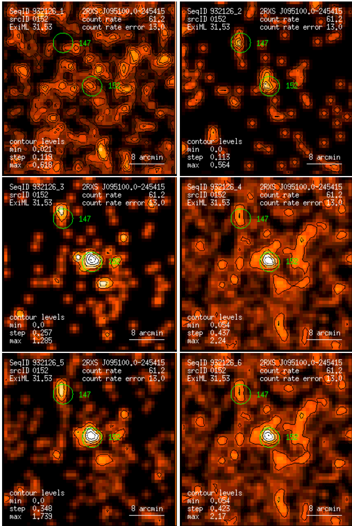
Figure 152: RASS 932126: detection 0152: band rate images, Gaussian filter: (1) PSPC channels 11 – 41, (2) 52 – 90, (3) 91 – 201, (4) 11 – 235, (5) 52 – 201, (6) 11 – 201. Broad band rates in counts/ks. Band rate contour levels in counts/ks/arcmin 2 .
