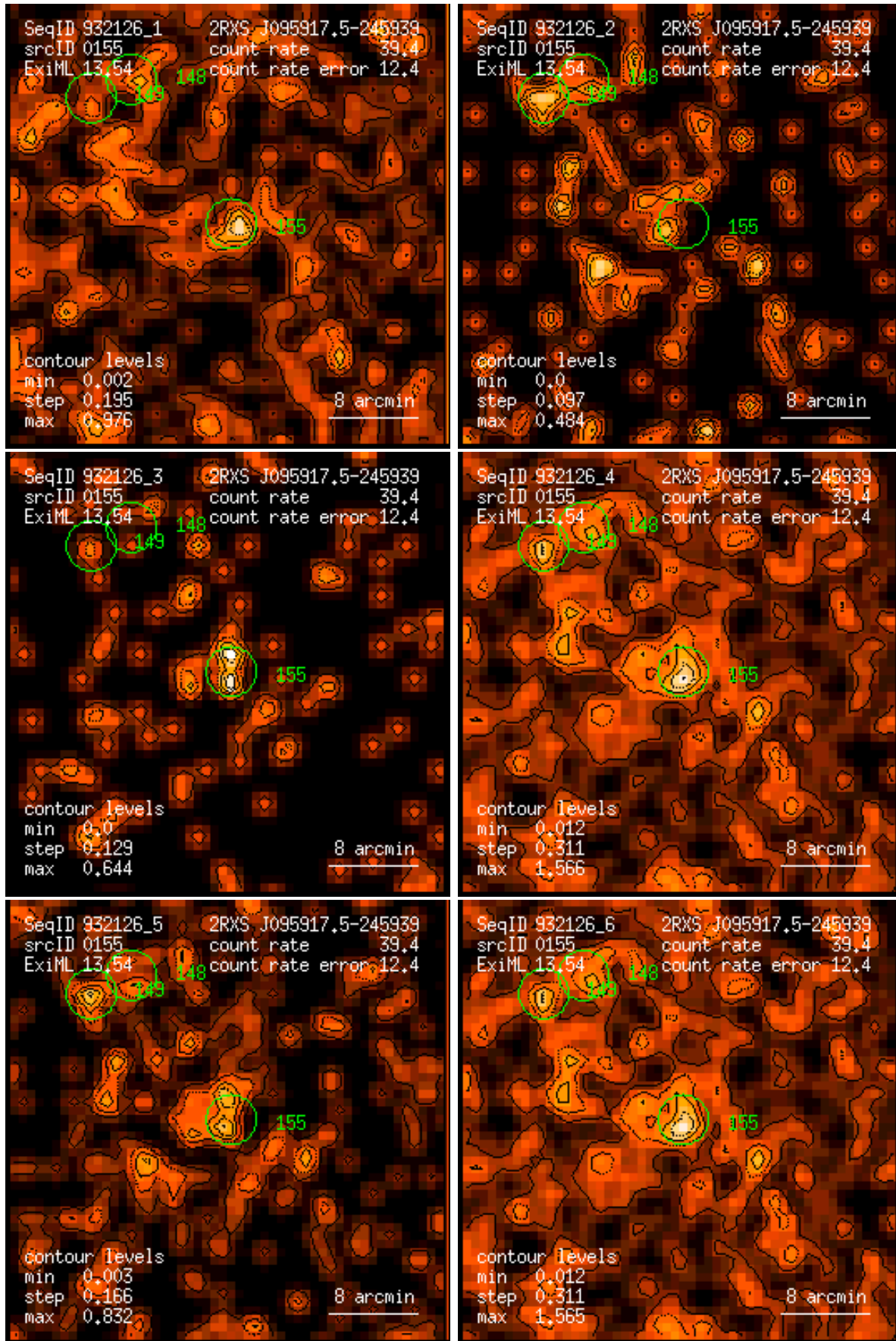
Figure 155: RASS 932126: detection 0155: band rate images, Gaussian filter: (1) PSPC channels 11 – 41, (2) 52 – 90, (3) 91 – 201, (4) 11 – 235, (5) 52 – 201, (6) 11 – 201. Broad band rates in counts/ks. Band rate contour levels in counts/ks/arcmin 2 .
