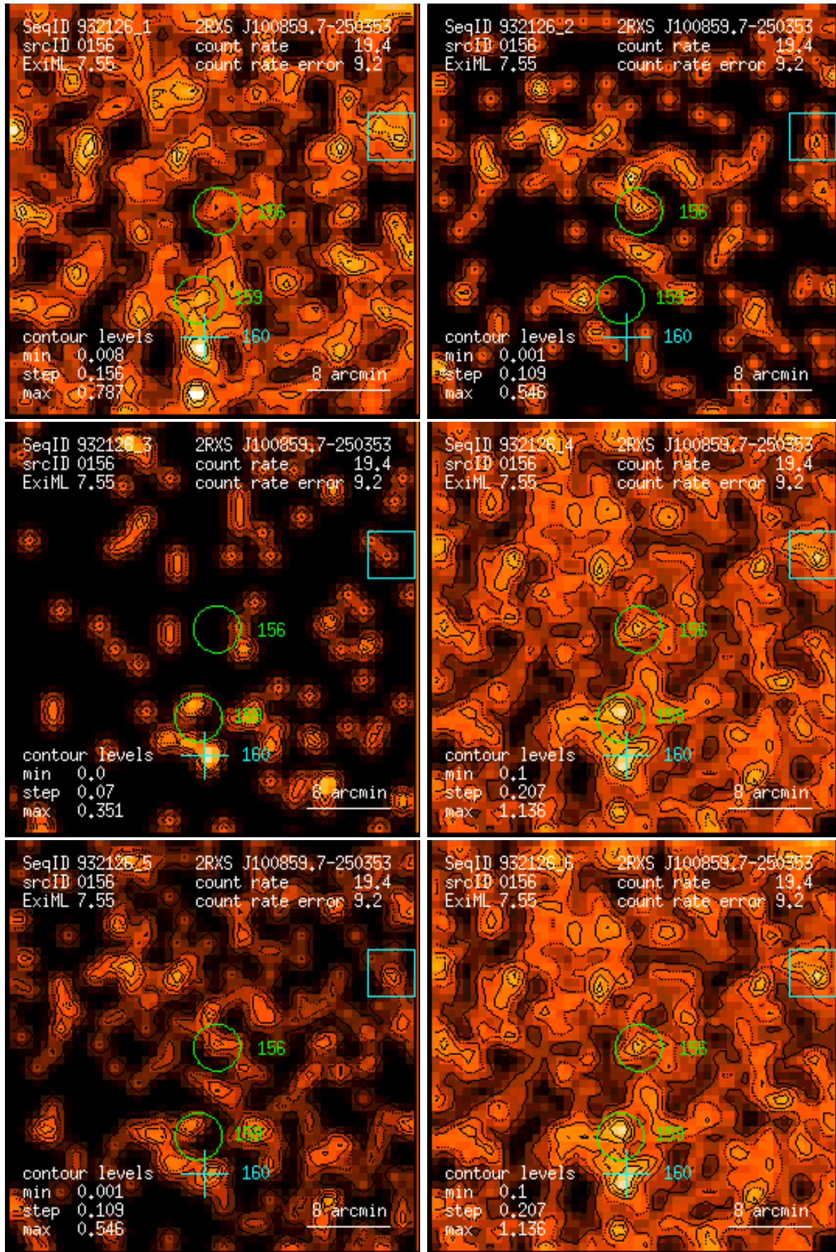
Figure 156: RASS 932126: detection 0156: band rate images, Gaussian filter: (1) PSPC channels 11 – 41, (2) 52 – 90, (3) 91 – 201, (4) 11 – 235, (5) 52 – 201, (6) 11 – 201. Broad band rates in counts/ks. Band rate contour levels in counts/ks/arcmin 2 .
