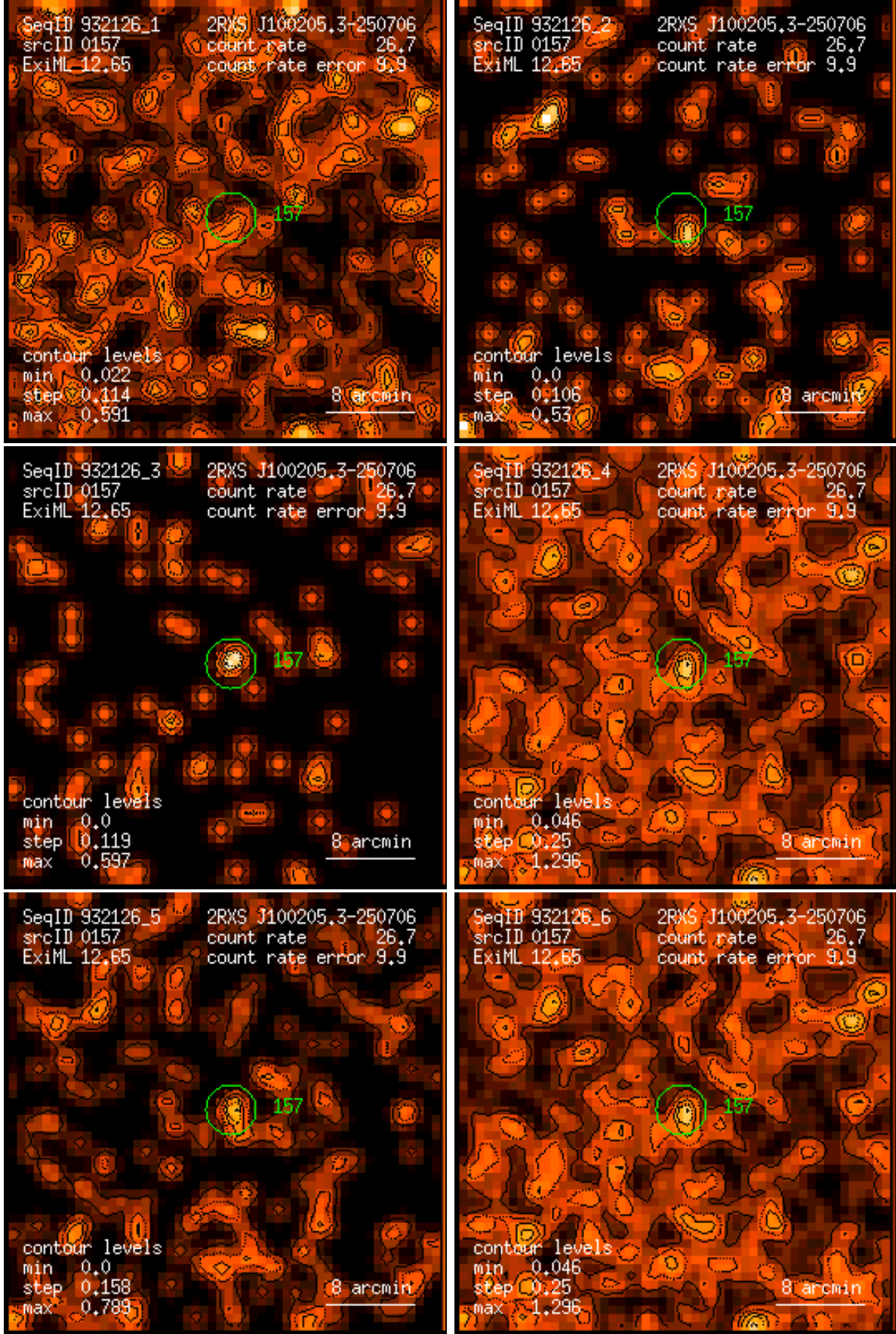
Figure 157: RASS 932126: detection 0157: band rate images, Gaussian filter: (1) PSPC channels 11 – 41, (2) 52 – 90, (3) 91 – 201, (4) 11 – 235, (5) 52 – 201, (6) 11 – 201. Broad band rates in counts/ks. Band rate contour levels in counts/ks/arcmin 2 .
