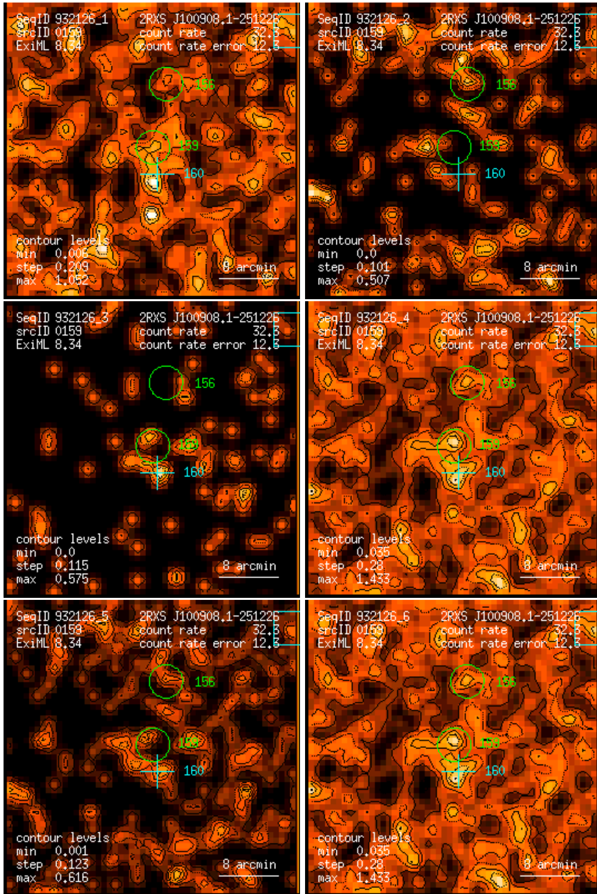
Figure 159: RASS 932126: detection 0159: band rate images, Gaussian filter: (1) PSPC channels 11 – 41, (2) 52 – 90, (3) 91 – 201, (4) 11 – 235, (5) 52 – 201, (6) 11 – 201. Broad band rates in counts/ks. Band rate contour levels in counts/ks/arcmin 2 .
